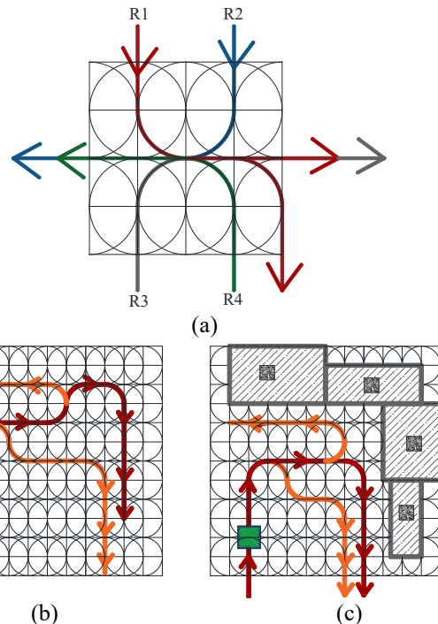
Figure. 6: Representation of route flows for transport and maintenance systems. a) Flexible route design, b) Flexible layout design, c) Flexible route design in an area with equipment and machinery. Source: The authors.
