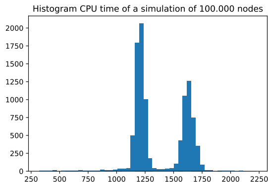
Figure 3.3: Histogram of the computation time of each one of the 10,100 realizations of the model using networks of 100,000 nodes. The average time is 1374.5 seconds, around 23 minutes.
