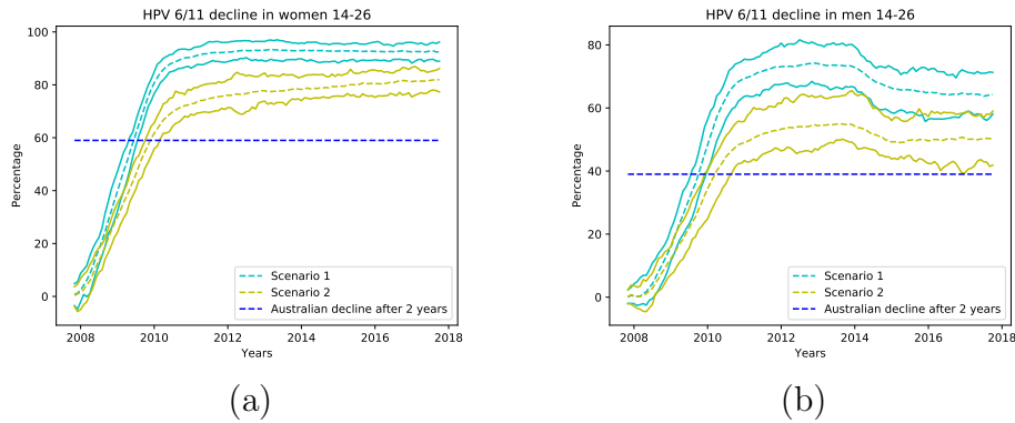
Figure 5.2: Percentage of decline of women (a) and men (b) aged 14-26 infected of LR HPV 6 and/or 11 (and consequently of genital warts) after the implementation of the vaccination program. The cyan lines correspond to the average and 95% confidence interval for Scenario 1 and the yellow lines to Scenario 2. After 2 years, the model shows a decline of 72% for Scenario 1 and 54.8% for Scenario 2, in average, for women and 38.9% for Scenario 1 and 27.7% for Scenario 2, in average, for men.
