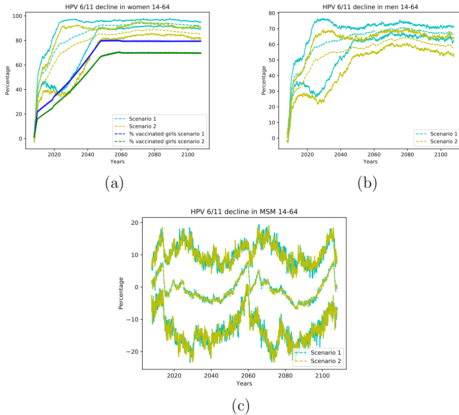
Figure 5.4: Percentage of decline of women (a), men (b) and MSM (c) aged 14-64 for the vaccination program in Australia. The cyan lines correspond to the average and 95% confidence interval for Scenario 1 and the yellow lines to Scenario 2. In the figure (a), blue and green lines correspond to women vaccination percentage for Scenario 1 and 2, respectively. Notice that the herd immunity effect contributes to the decline in the number of infections in men and the decline in the number of infections for unvaccinated women. This latter can be seen when the decline lines are over the vaccination line. However, any herd immunity effect can be seen in MSM.
