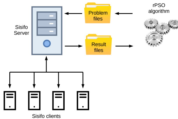
Figure 3.1: Introduction of the asynchronous rPSO algorithm in the Sisifo environment. rPSO manages the generation of new problems and put them in the Problem files folder and the reading and processing of the solution files located in the Result files folder.
