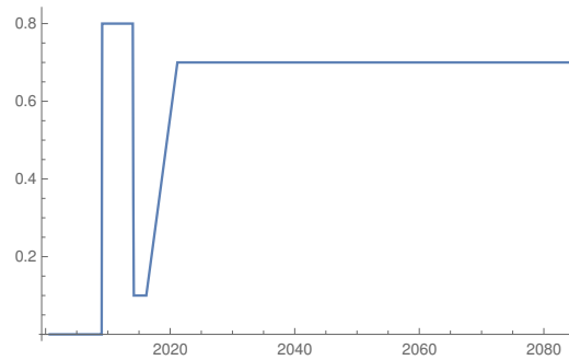
Figure 6.10: Evolution of the HPV vaccine coverage in Denmark from the program starting in 2009.
