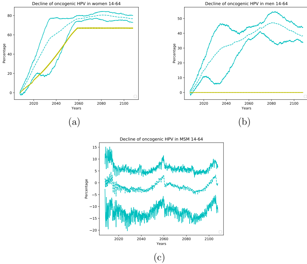
Figure 6.2: Decline of HPV oncogenic HR infections in 14-64 years old women, men and MSM over the time, from Oct 2007, when the vaccination campaign started in Spain. In the women decline, we include the percentage of vaccinated women. It helps to visualize the herd immunity effect when the decline line is over the vaccination line. In case of men, the lines over the yellow abscissa line means effect of the herd immunity. For the MSM, there is not herd immunity effect.
