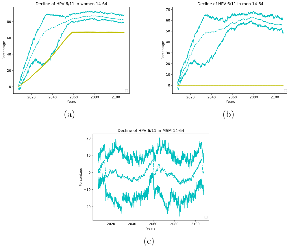
Figure 6.1: Decline of HPV LR 6/11 infections, and consequently, of genital warts (GW) in 14-64 years old women (a), men (b) and MSM (c) over the time, from Oct 2007 when the vaccination campaign started in Spain. In the women decline, we include the percentage of vaccinated women. It helps to visualize the herd immunity effect when the decline line is over the vaccination line. In case of men, the lines over the yellow abscissa line means effect of the herd immunity. However, for the MSM, as in the Australian case, there is not herd immunity effect.
