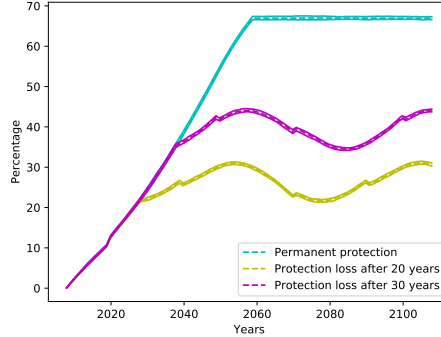
Figure 6.7: Percentage of women protected by the vaccine in three scenarios: permanent protection (cyan line), total loss of protection after 30 years (magenta line) and total loss of protection after 20 years (yellow line).
