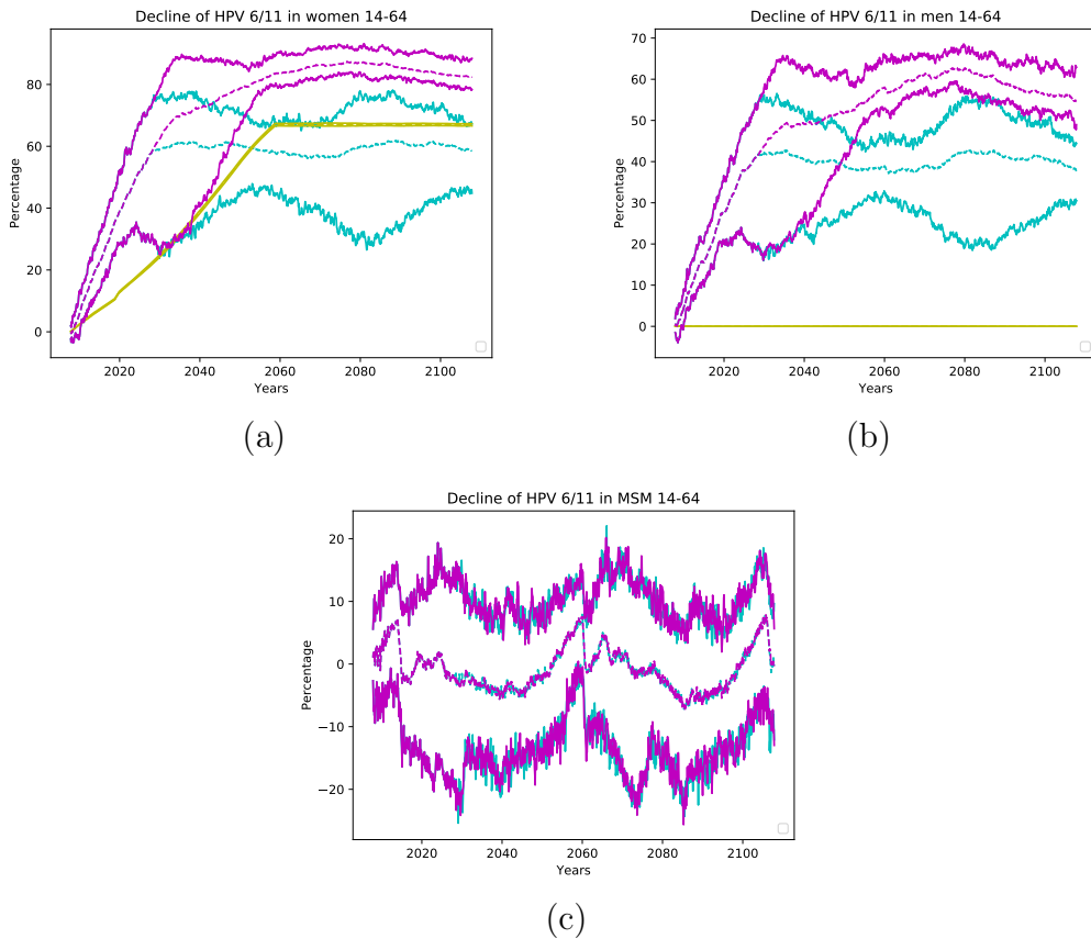
Figure 6.4: Comparative of the decline of HPV LR 6/11 in 14-64 years old women (a), men (b) and MSM (c) over the time, between the scenario where the effect of the vaccine is permanent (magenta lines, representing the mean and the 95% confidence interval) and the scenario where the effect of the vaccine disappear completely after 20 years (cyan lines, representing the mean and the 95% confidence interval). As we can see, for women and men, the latter stabilizes in levels of decline about 20% less, in average, than the case where the vaccine protects permanently. For MSM there are not changes between both scenarios.
