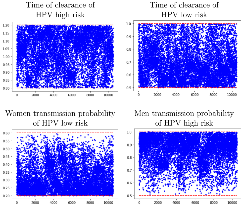
Figure 3.2: Upper figures: Time of clearance of HPV high risk and low risk, both for men and women. Lower figures: on the left, probability to transmit low risk HPV if the infected is a woman; on the right, probability to transmit high risk HPV if the infected is a man. Red dashed lines correspond to the bounds of each parameter. We can see that most of the search space is explored in all the cases.
