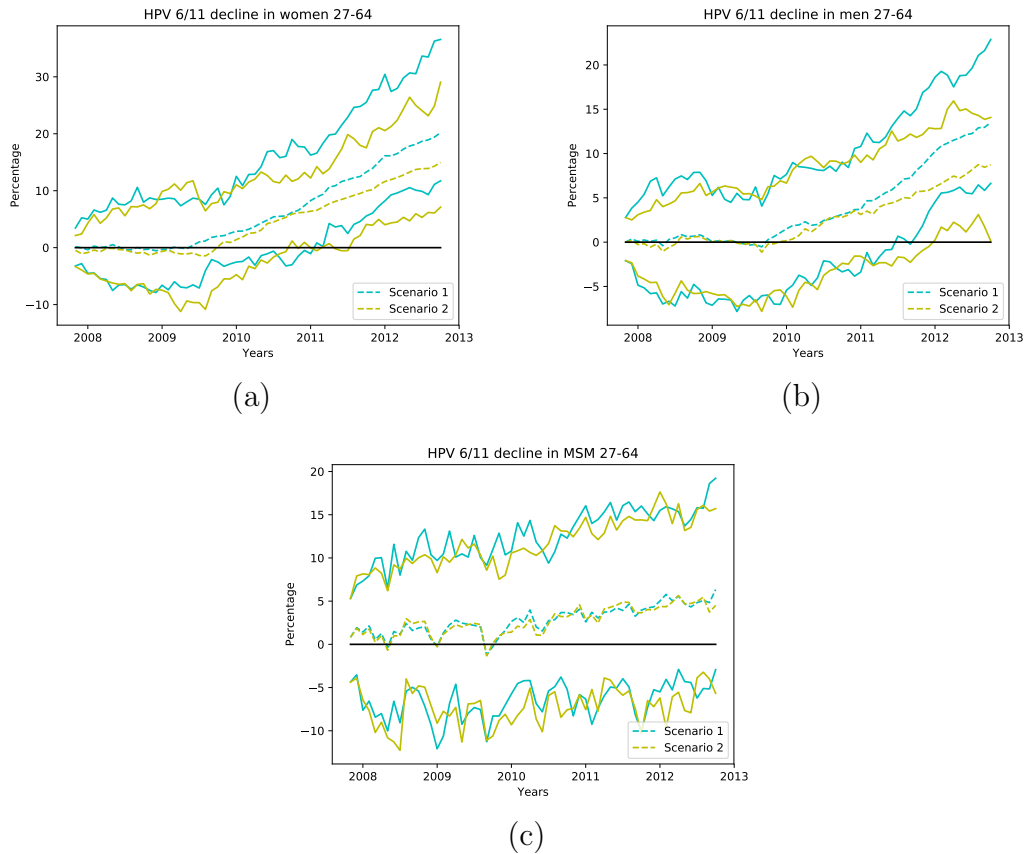
Figure 5.3: Percentage of decline of women (a), men (b) and (c) MSM aged 27-64 infected of LR HPV 6 and/or 11 (and consequently of genital warts) after the implementation of the vaccination program in both scenarios. The cyan lines correspond to the average and 95% confidence interval for Scenario 1 and the yellow lines to Scenario 2. Notice that, in average, no significant decline appears in the 5 years after the implementation of the vaccination program.
