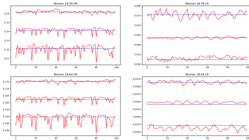
Figure 3.7: Means and 95% confidence intervals of the 30 selected realizations (in red) compared to the means and 95% confidence intervals of the data (blue).
