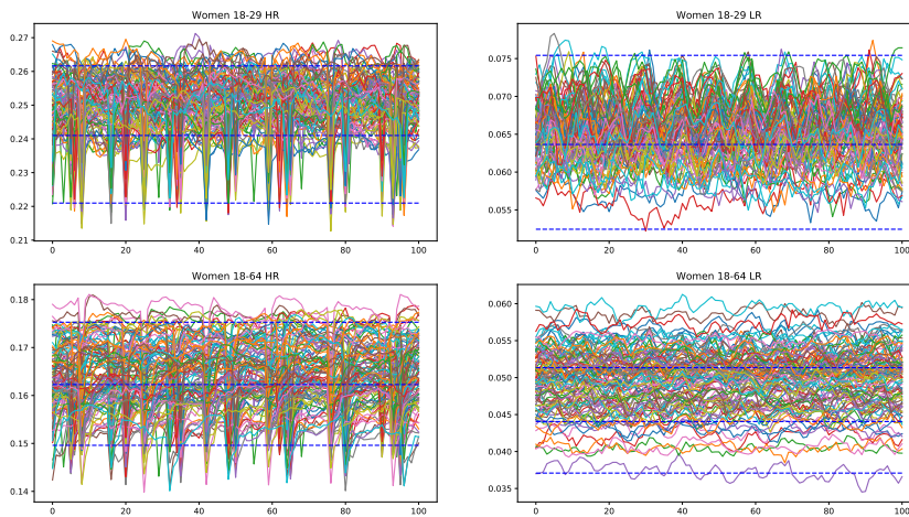
Figure 3.4: Drawing of the 100 model realizations with error less than 0.01 from month 400 to 499.
