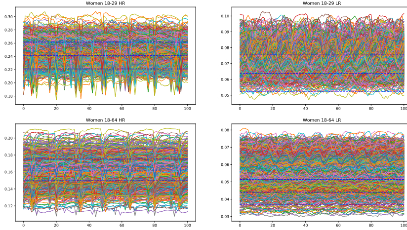
Figure 3.5: Drawing of the 1282 model realizations with error less than 0.05 from month 400 to 499. These realizations cover the 95% confidence intervals of the data, represented by the blue horizontal dashed lines.
