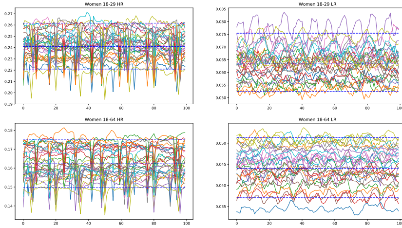
Figure 3.6: Drawing of the 30 selected model realizations from month 400 to 499. These realizations are the ones whose means and 95% confidence intervals resemble the most the data in Table 3.1, represented by the blue horizontal dashed lines.
