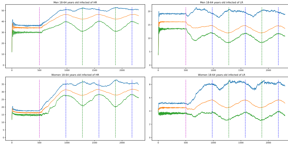
Figure 4.3: Mean and 95% confidence intervals of the prevalence for 18-64 men and women for HR and LR. Vertical dashed lines indicate milestones of interest. Note the oscillations of the prevalence levels. The blue and green vertical lines correspond to the peaks and valleys of the oscillations. The magenta line, points the month 500 when dynamic network starts.
