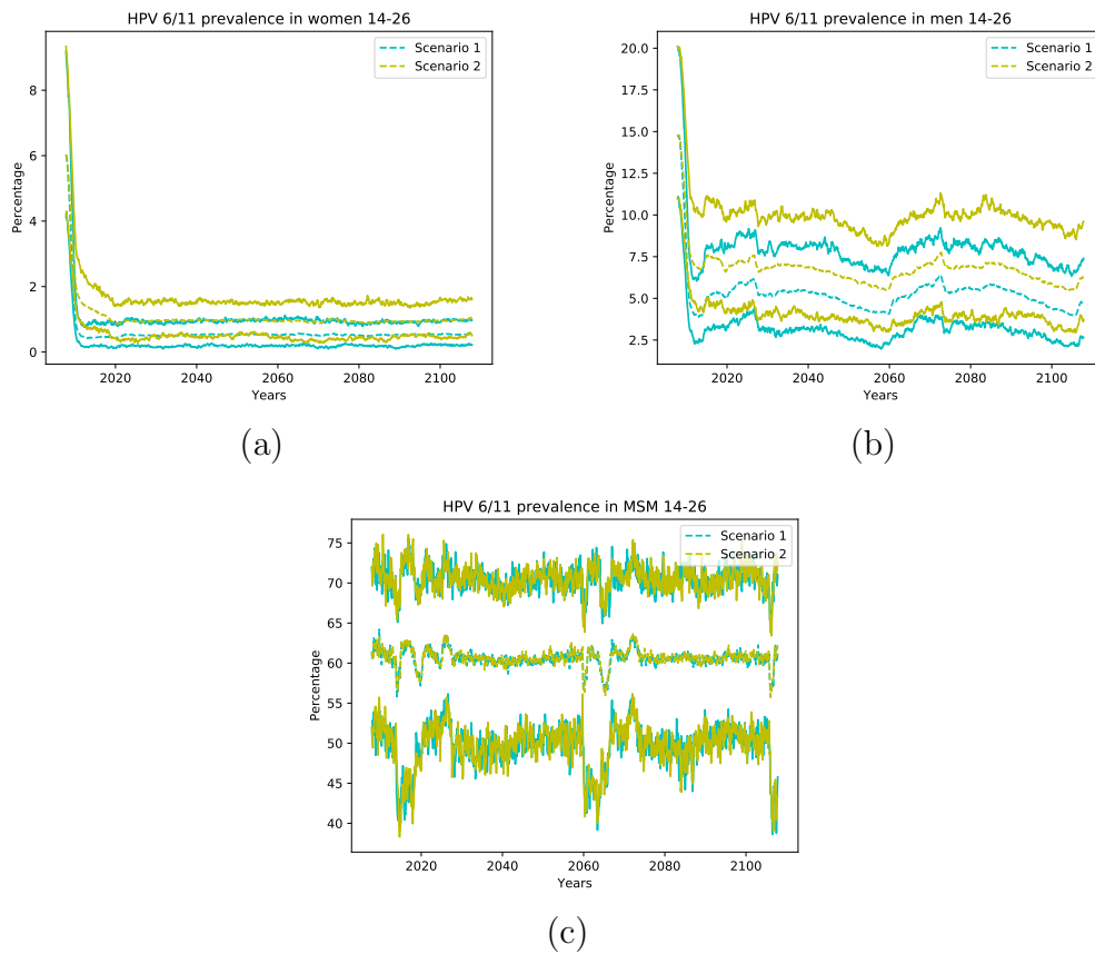
Figure 5.1: Percentage of women (a), men (b) and MSM (c) aged 14-26 infected of LR HPV 6 and/or 11 after the implementation of the vaccination program. The cyan lines correspond to the average and 95% confidence interval for Scenario 1 and the yellow lines to Scenario 2. We can see the fast decrease for women and men in both scenarios from the very beginning. However, there is not effect on MSM.
