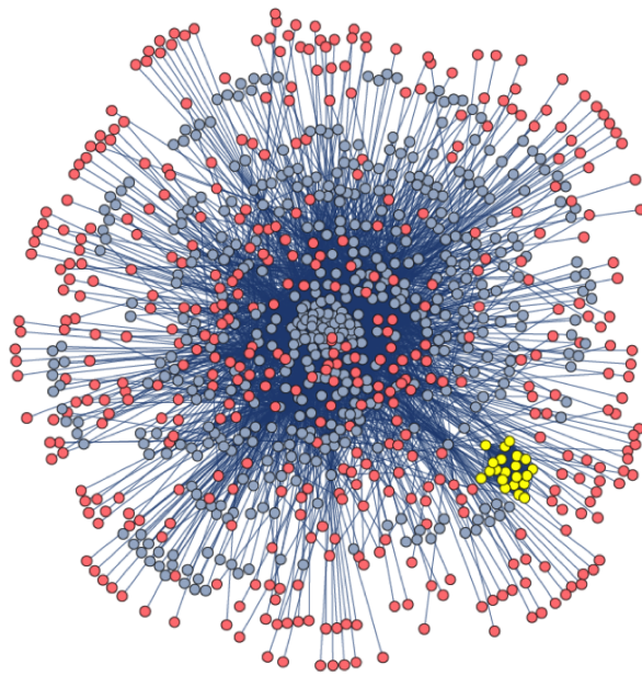
Figure 1.4: Example Network of 1,000 nodes, MSM in yellow, women in red and men in blue.
