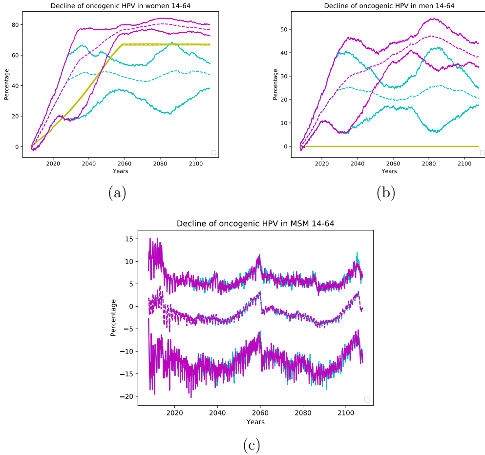
Figure 6.5: Comparative of the decline of oncogenic HPV infections in 14-64 years old women (a), men (b) and MSM (c) over the time, between the scenario where the effect of the vaccine is permanent (magenta lines, representing the mean and the 95% confidence interval) and the scenario where the effect of the vaccine disappear completely after 20 years (cyan lines, representing the mean and the 95% confidence interval). The graphs are very similar to the ones in Figure 6.4 with the only change that the difference between the levels of decline are higher. For MSM there are not changes between both scenarios.
