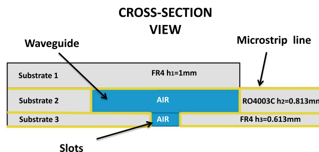
Figure 2. Cross-section view of the selected layer stack-up.
