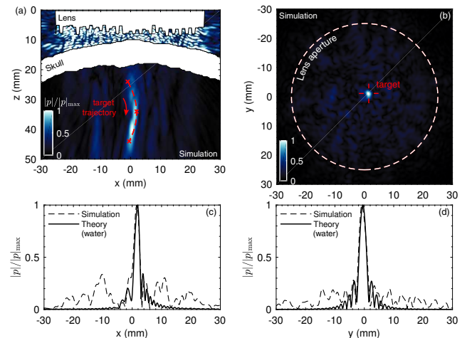
FIG. 8. Simulation results for the self-bending holographic beam designed for a realistic skull. (a) Axial cross-section of the pressure distribution at y = 0 mm. (b) Transversal cross-section at z = 35 mm. (c) Lateral cross-section at z = 35 mm and y = 0 mm. (d) Lateral cross-section at z = 35 mm and x = 2 mm.
