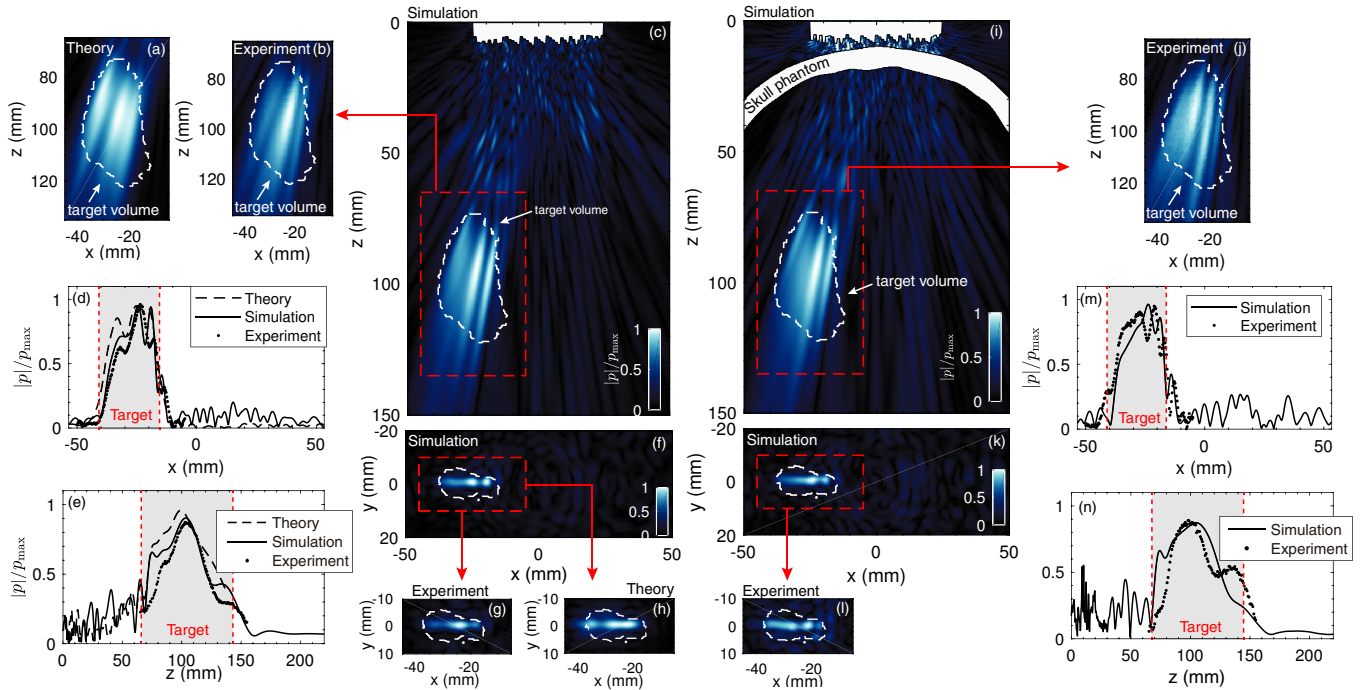
FIG. 6. Volumetric hologram results. (a,b,c) Theoretical, experimental and simulated axial pressure distribution in water. (d,e) Transversal and axial field cross-sections in water. (f,g,h) Simulated, experimental and theoretical transversal field distribution in water. (i,j) Simulated and experimental axial pressure distribution including the skull phantom. (k,l) Corresponding transversal pressure distribution and (m,n) transversal and axial cross-section, respectively.
