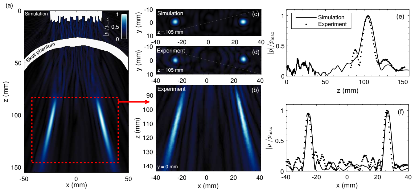
FIG. 4. Axial field cross-section obtained for the bifocal lens using simulations (a) and experiments (b). (c-d) Corresponding transversal pressure field distributions. Colorbar in units normalized to the peak pressure. (e,f) Simulated and experimental normalized axial and transversal field cross-sections, respectively.
