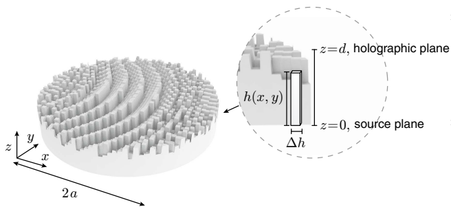
FIG. 3. Geometry of the holographic lens. The lens, of aperture 2a is subdivided in pixels of height h(x, y) . The source is located at z = 0 , while the holographic plane is located at z = d .
