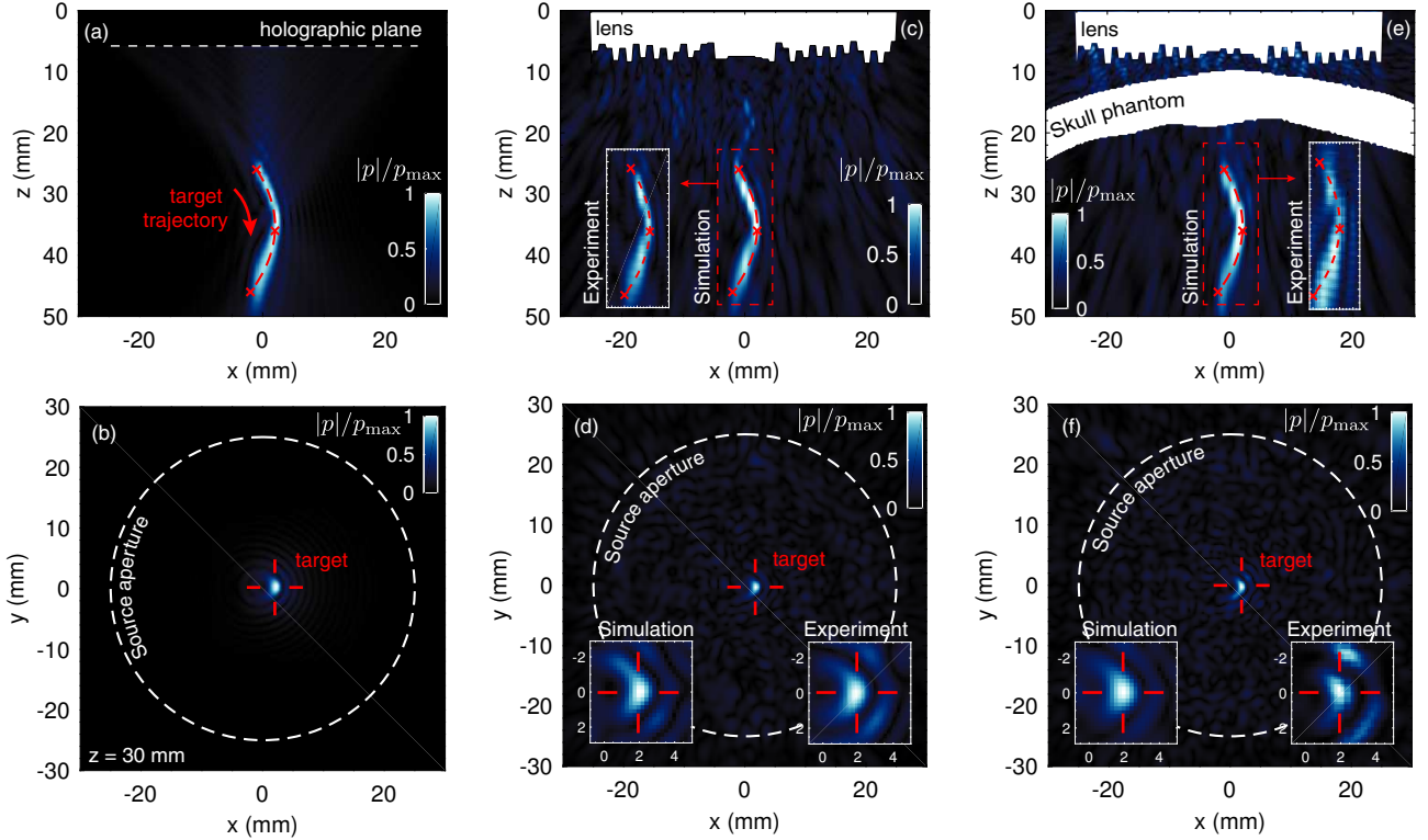
FIG. 5. Theoretical (a) axial and (b) transverse pressure field distribution for the self-bending beam in water. Simulated (c) axial and (d) transverse pressure field distribution for the self-bending beam in water. Corresponding experimental results are shown in the insets in (c) and (d). (e,f) Simulated axial and transversal pressure field including the skull phantom. Corresponding experimental results are shown in the insets in (e) and (f).
