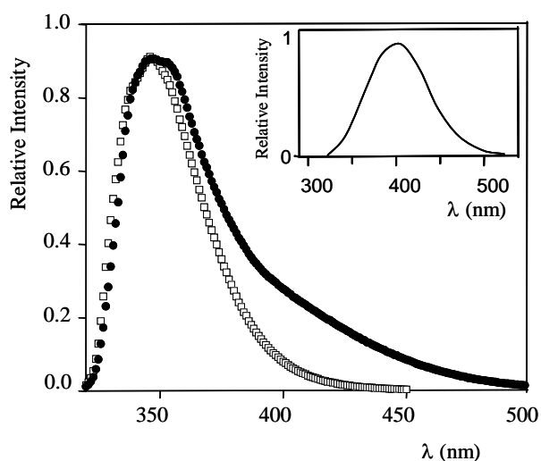
Figure 4. Normalised fluorescence spectra of ( S )-NPX (□), and the model dyad (●) in acetonitrile ( \lambda_{\text{exc}} = 266 nm). Insert: fluorescence spectrum of the excimer obtained by difference between the normalised spectra of S -NPX and that of the model dyad.
