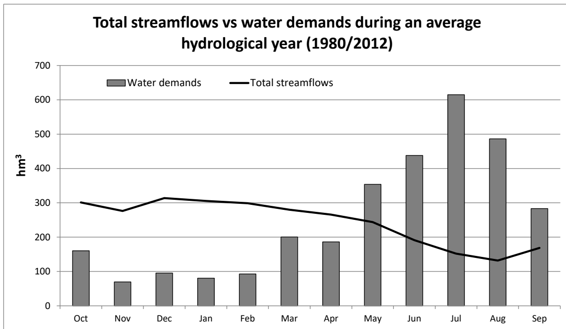
Figure 2 | Total streamflows VS water demands during an average hydrological year (1980/2012) for the Jucar River Basin district.
