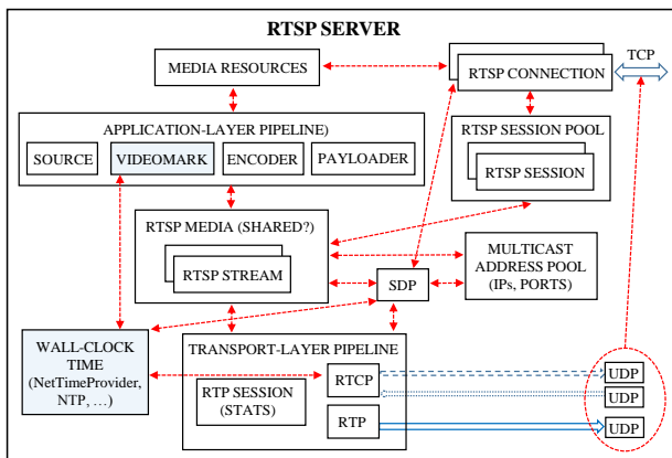
Figure 1. Server Architecture.
