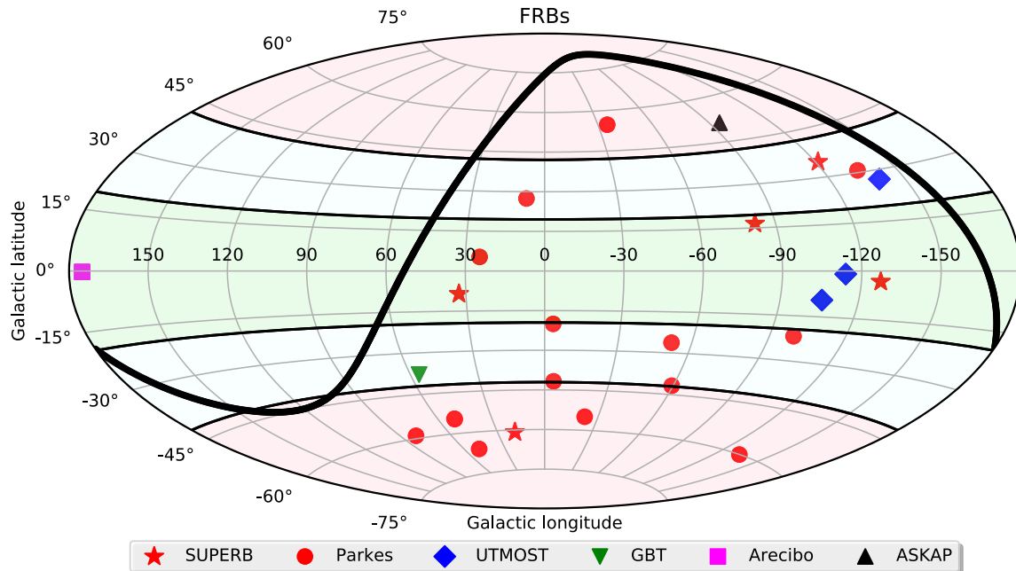
Figure 4. An Aitoff projection of the sky distribution of all published FRBs. The shaded regions show the three Galactic latitude bins in Table 5. The bold black line shows the horizon limit of the Parkes radio telescope.
