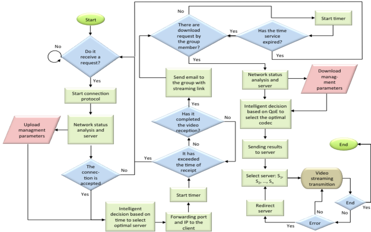
Figure 2: Intelligent manager algorithm in IMS application level.
