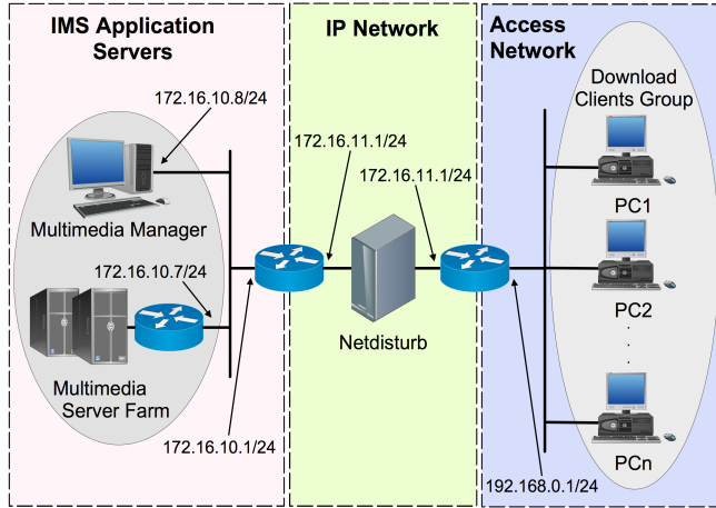
Figure 3: Network topology.
