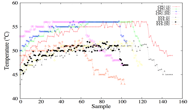
Figure 6: Impact of connected users on the system temperature.
