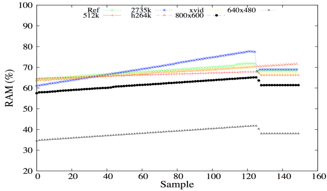
Figure 8: Impact of transcoding on the system memory.
