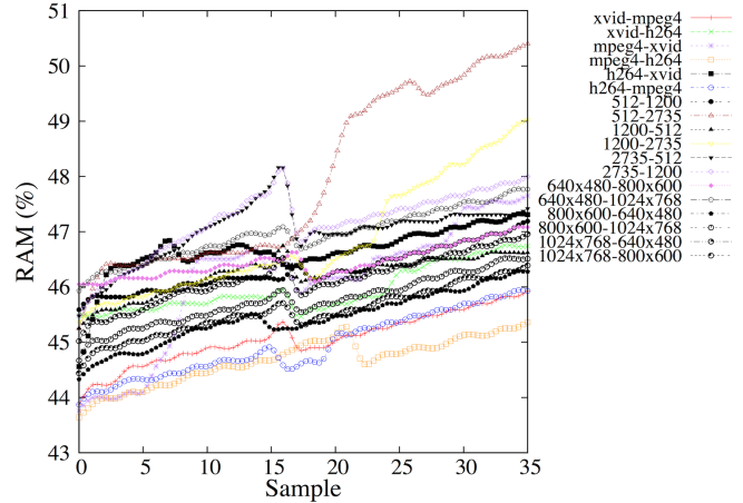
Figure 11: Impact of dynamic transcoding on the memory.
