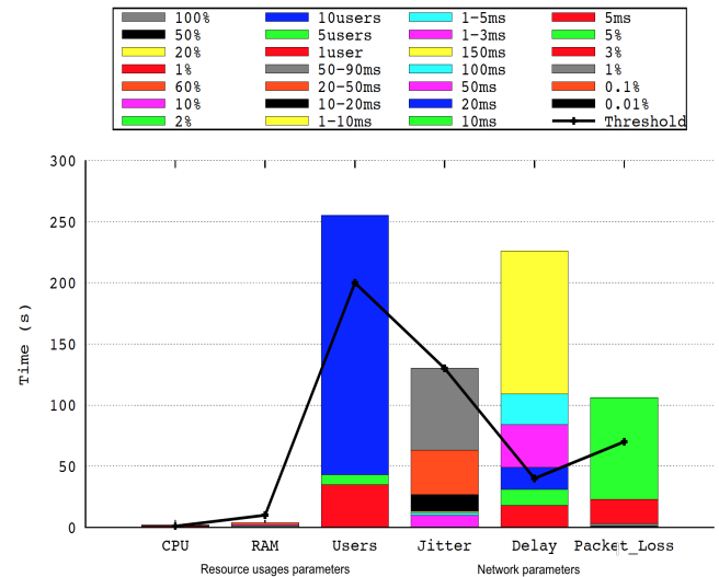
Figure 4: Evaluate the threshold values.
