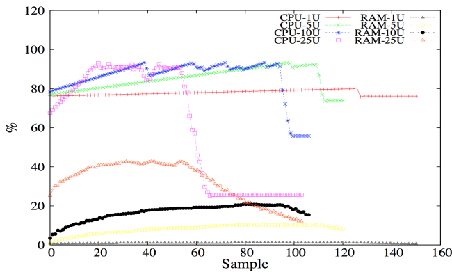
Figure 5: Impact of connected users on the system resources.
