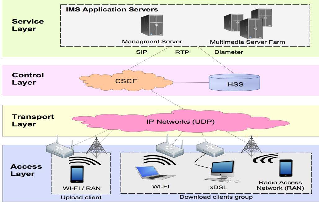
Figure 1: The IMS architecture proposal.
