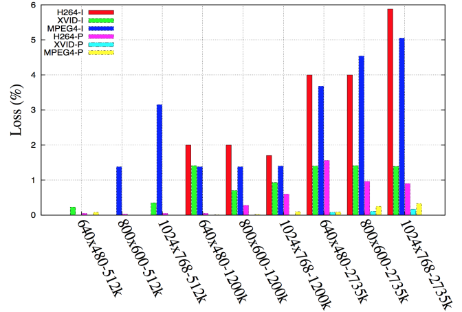
Figure 17: Impact of GOP on the QoE
