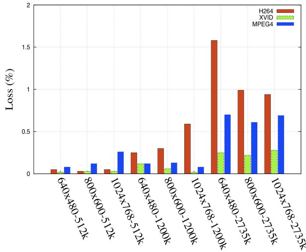
Figure 16: Frames lost for different codecs.
