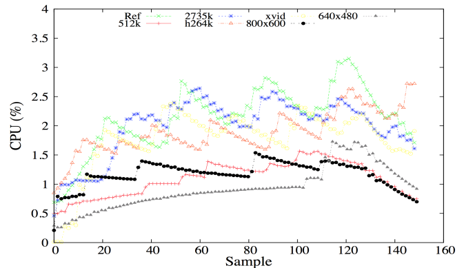
Figure 7: Impact of transcoding on the system CPU.
