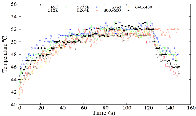
Figure 9: Impact of transcoding on the system temperature.
