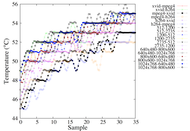
Figure 12: Impact of dynamic transcoding on the temperature.
