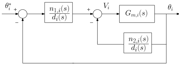
Figura 9: Control PID.
