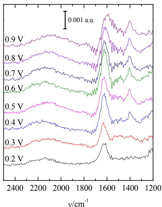
50 51 Figure 7. FTIR for the adsorbed species on the Pt(111) electrode in solutions containing 0.1 M HClO 4 52 10 mM citric acid (pH=1.2) for different electrode potentials. 53 54 55 56 57
