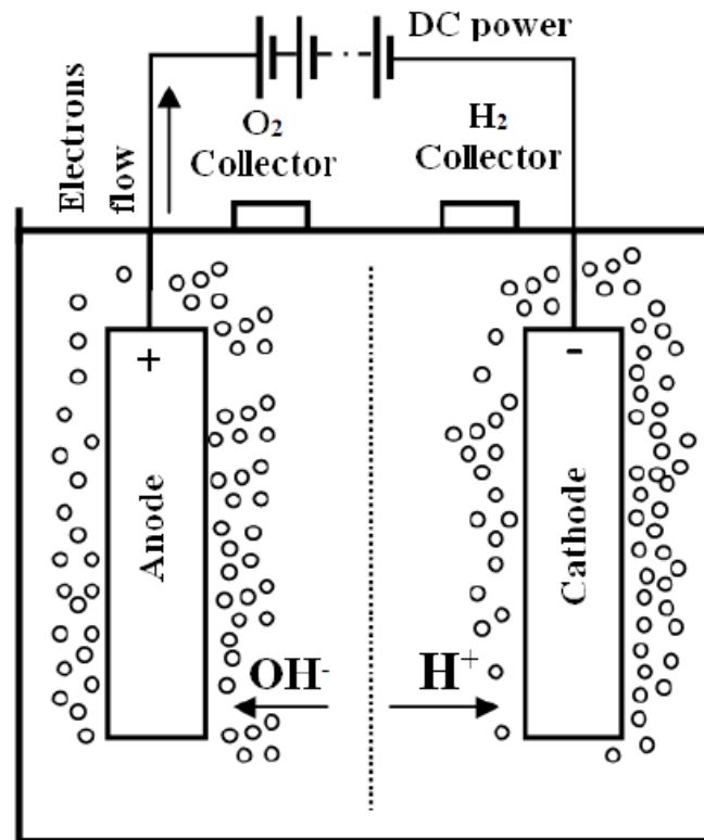
Figure 6. Schematic operation of electrolysis
