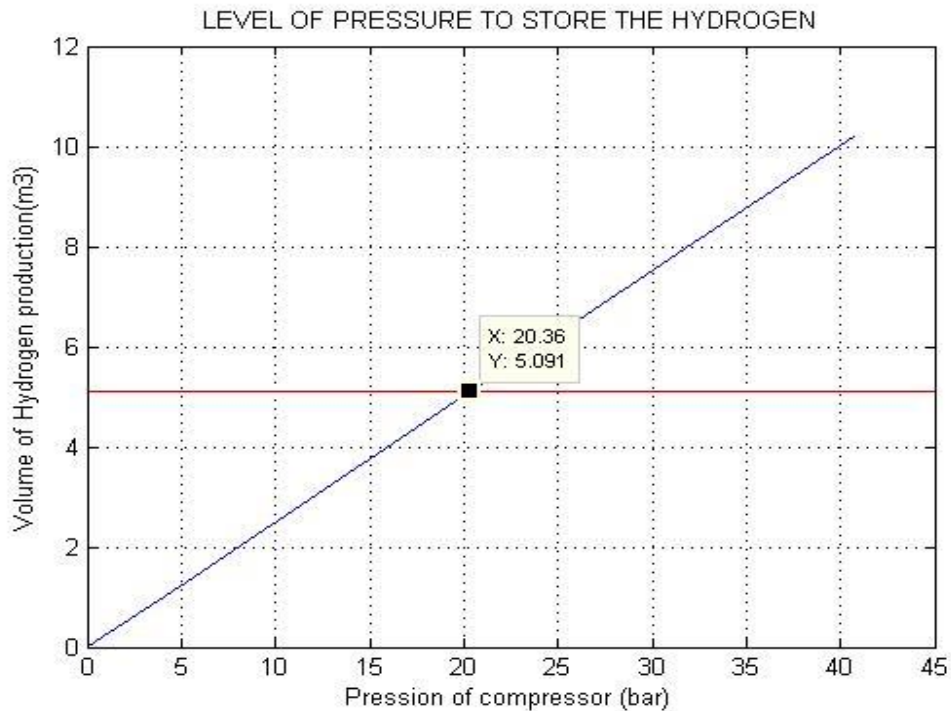
Figure 14. Level of pressure to store the hydrogen
