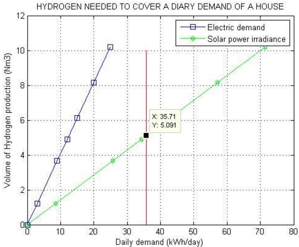
Figure 13. Hydrogen needed to cover a daily demand of a house
