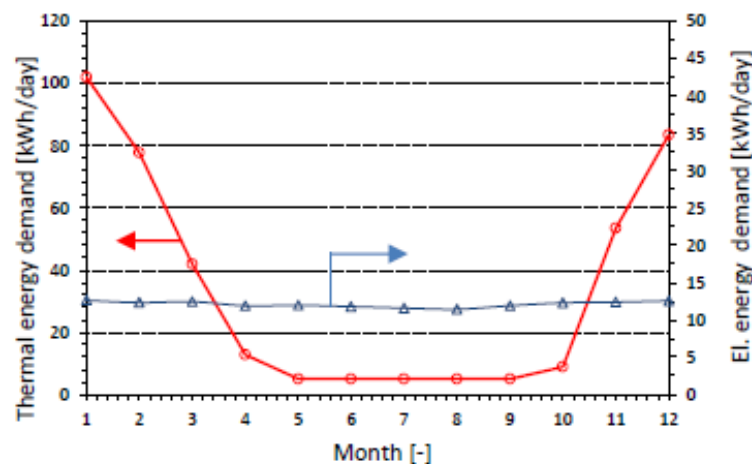
Figure 11. Daily electrical and thermal energy monthly profile.
