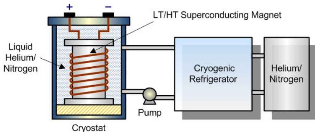
Figure 3. Electromagnetic storage scheme.
