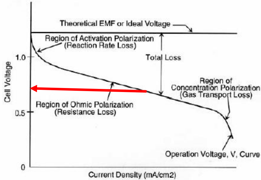
Figure 9. Cell polarization curve.
