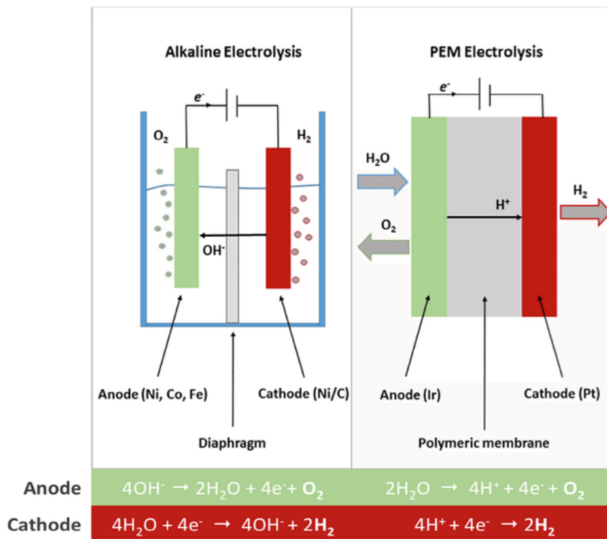
Figure 7. Comparative scheme between alkaline and PEM electrolysis.
