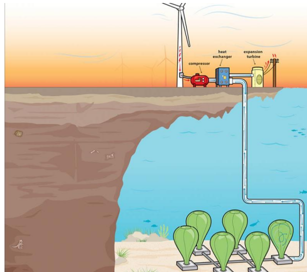
Figure 2. Compression storage scheme
