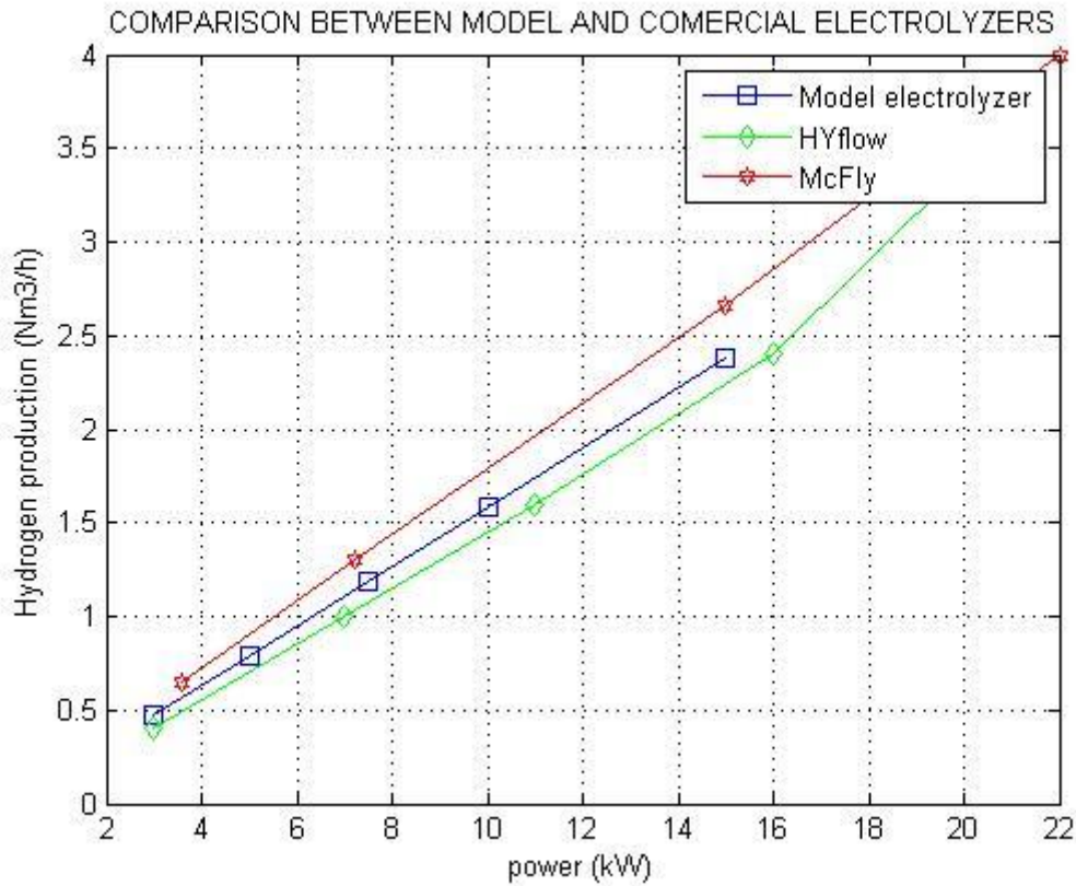
Figure 10. Comparison between model and commercial electrolyzers.
