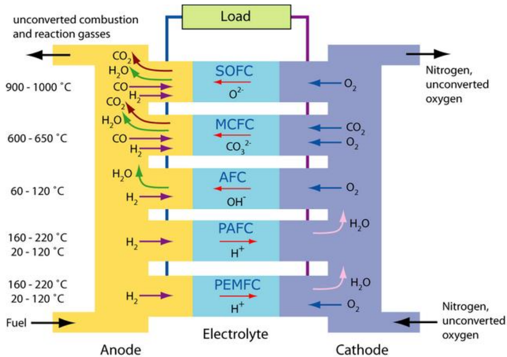
Figure 8. Types of Fuel Cells
