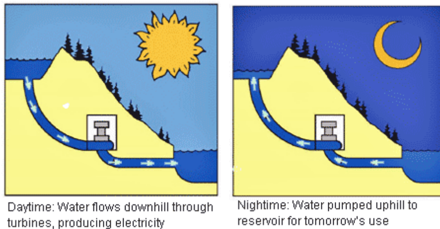
Figure 1. Hydroelectric scheme during the day.
