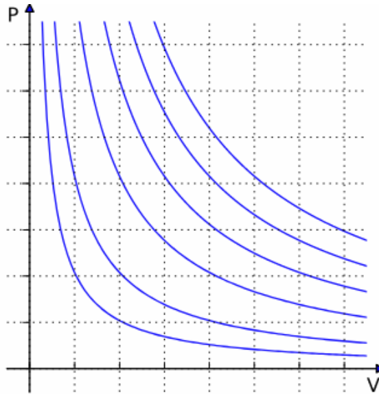
Figure 12. Isotherms of an ideal gas.
