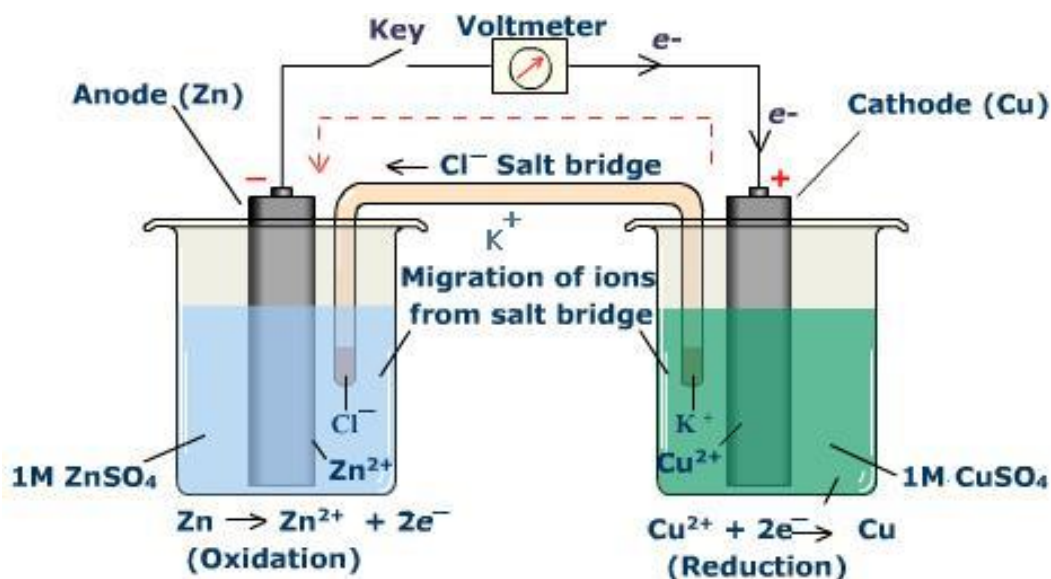
Figure 4. Battery diagram of working.
