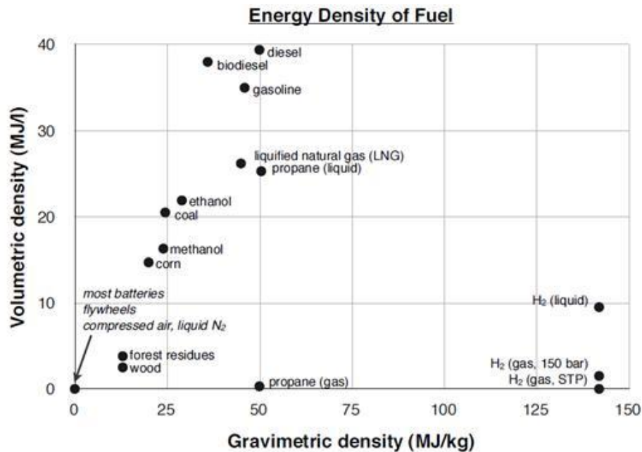
Figure 5.. Energy density of Fuel
