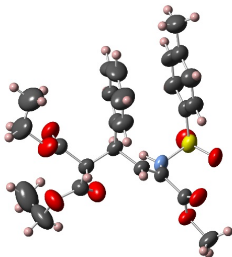
Figure 2. ORTEP plot for the X-ray structure of 3bl . The thermal ellipsoids are drawn at the 50% probability level.
