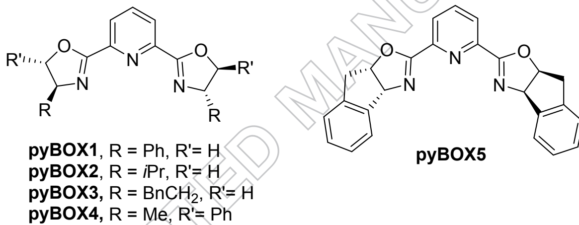
Figure 1. pyBOX-type ligands used in this study.
