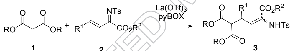
Scheme 1. Conjugate addition of malonate esters to N -tosyl imines derived from \beta,\gamma -unsaturated \alpha -keto esters.
