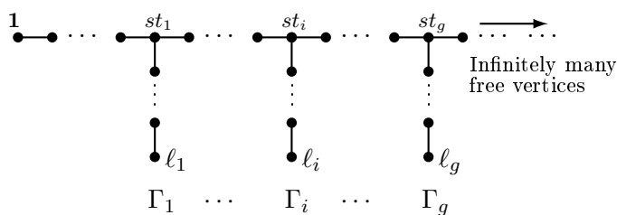
FIGURE 4. Dual graph of a curve valuation
