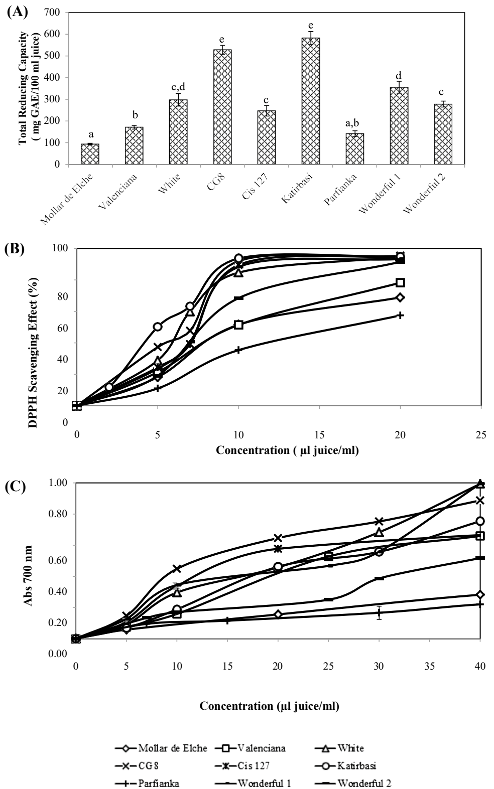
Fig. 2 Antioxidant activity of juice of nine pomegranate cultivars grown in Spain: Total Reducing Capacity (a), DPPH radical-scavenging activity (%) versus concentration of juice (b) and Reducing Power (Abs 700 nm) versus concentration of juice (c)
