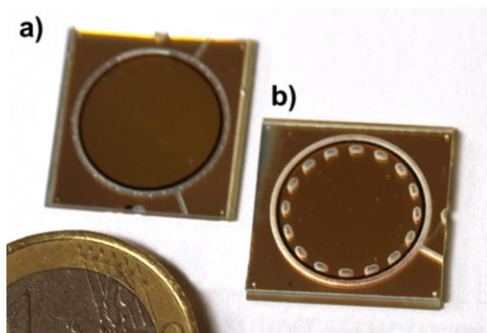
Fig. 6. Packaged devices after wafer scale fabrication and dicing: (a) UV and (b) \text{NO}_2 sensing chips.
