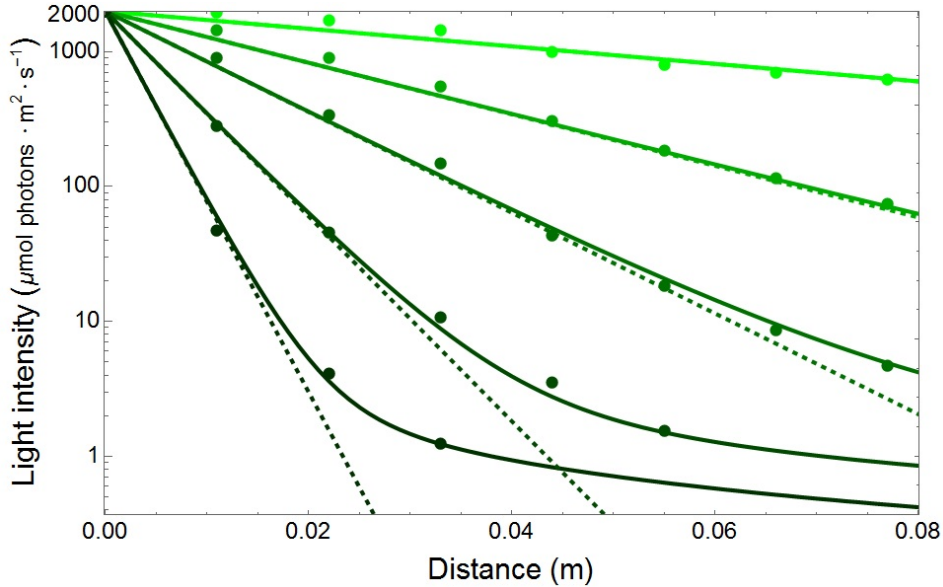
Figure 1: Light attenuation profiles of Synechocystis WT strain cultures exposed to 2000 \mu\text{mol photons} \cdot \text{m}^{-2} \cdot \text{s}^{-1} of white LED light at five different \text{OD}_{750} concentrations (0.1, 0.5, 1.0, 2.5 and 5.0) are depicted. Dots are the original source samples [8] and lines the modelling outcome (dashed lines Lambert-Beer law, solid lines Mittag-Leffler function). Darker colours correspond to denser suspensions.
