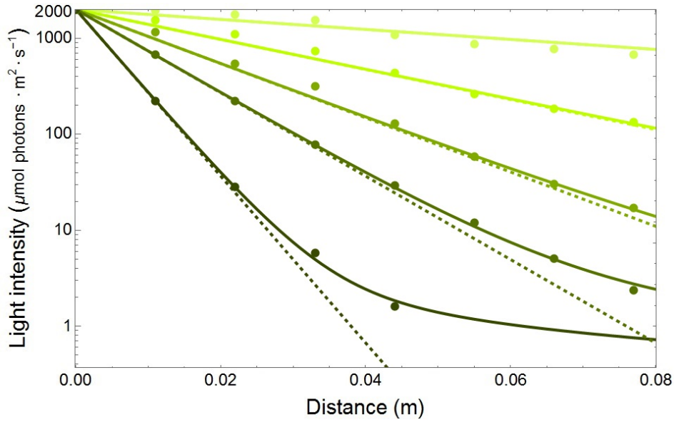
Figure 2: Light attenuation profiles of Synechocystis Olive strain cultures exposed to 2000 \mu\text{mol photons} \cdot \text{m}^{-2} \cdot \text{s}^{-1} of white LED light at five different \text{OD}_{750} concentrations (0.1, 0.5, 1.0, 2.5 and 5.0) are depicted. Dots are the original source samples [8] and lines the modelling outcome (dashed lines Lambert-Beer law, solid lines Mittag-Leffler function). Darker colours correspond to denser suspensions.
