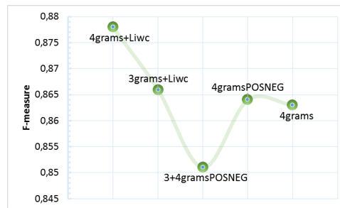
Fig. 2. Ranking of the 5 most effective features.
