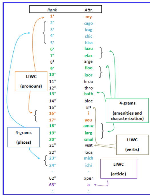
Fig. 4. Most discriminative features for positive reviews.
