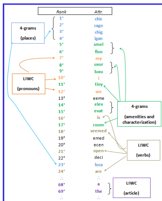
Fig. 3. Most discriminative features for negative reviews.
