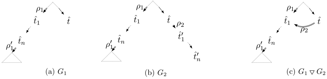
Figure 3: The graph widening behavior.
