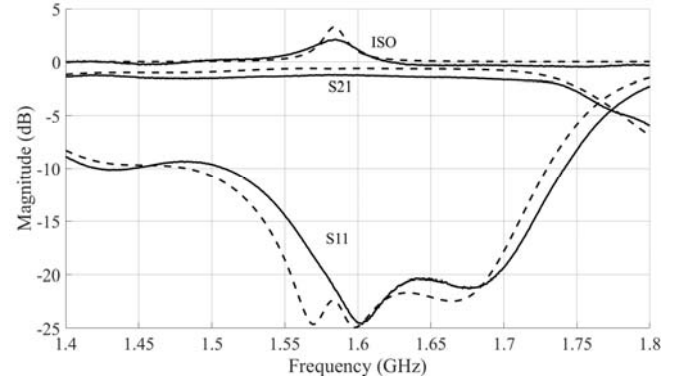
Fig. 10. Frequency responses (S-parameters and isolation) of the L-FTD with magnetized ferrites: simulated data (dashed lines) versus measurements (solid lines).
