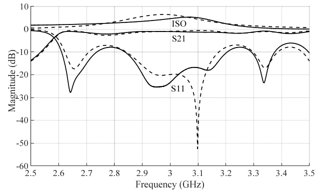
Fig. 11. Frequency responses (S-parameters and isolation) of the S-FTD with magnetized ferrites: simulated data (dashed lines) versus measurements (solid lines).
