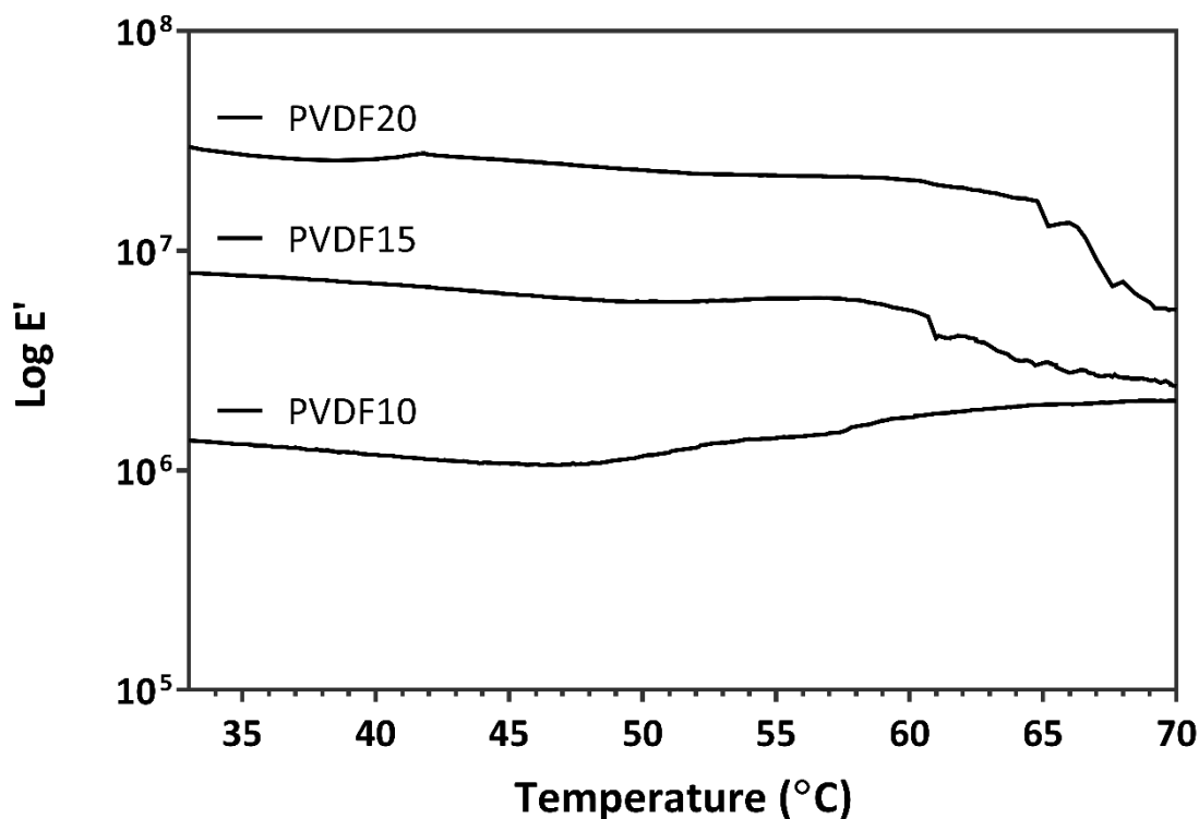
Figure 3. Storage modulus of PVDF membranes.
