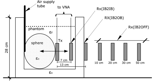
Fig. 1. Measurement elements setup.
