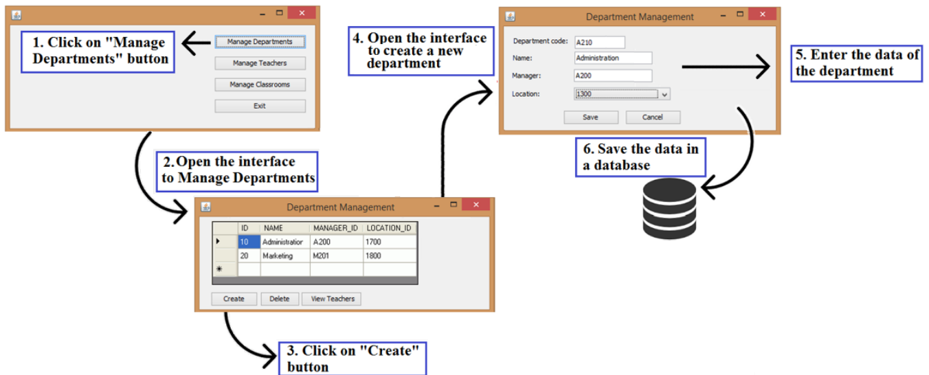
Figure 4. Software system supporting traditional interaction
