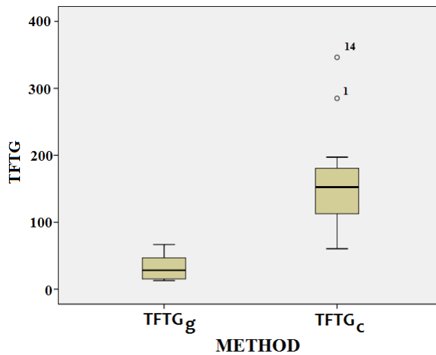
Figure 10. Box-plot of TFTG
