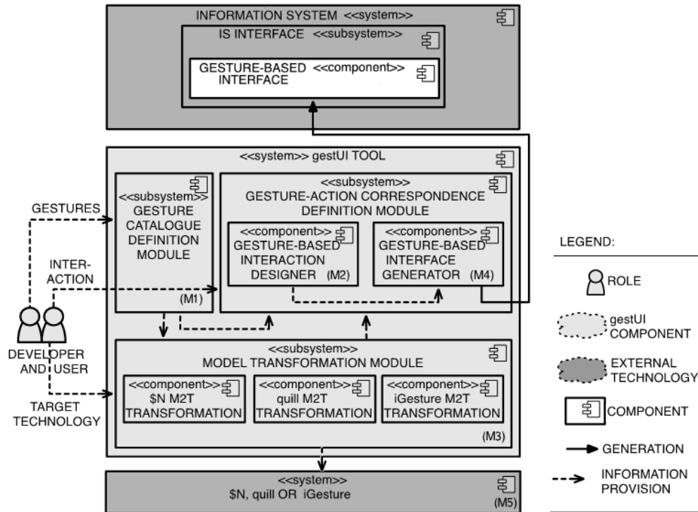
Figure 3. gestUI tool support
