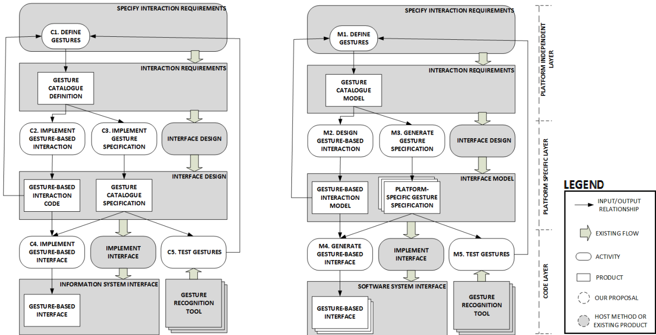
Figure 1. Methods overview: code-centric (left) and model-driven (gestUI) method (right)
