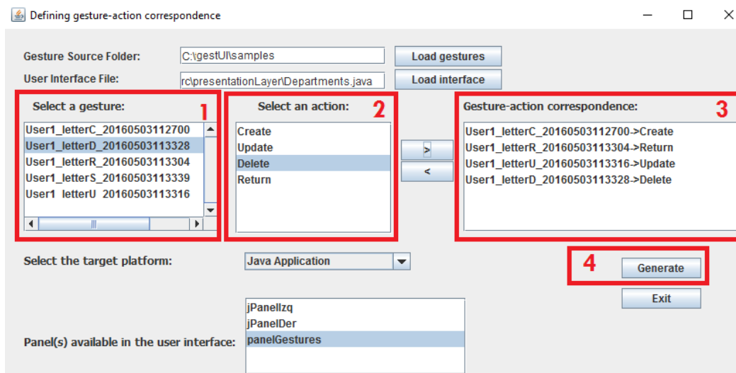
Figure 6. Gesture-action correspondence definition using tool support
