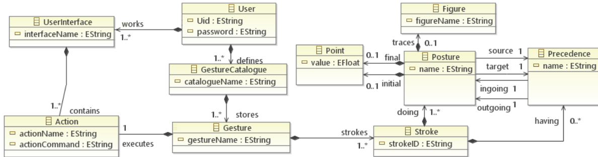
Figure 2. gestUI metamodel (Taken from [42])
