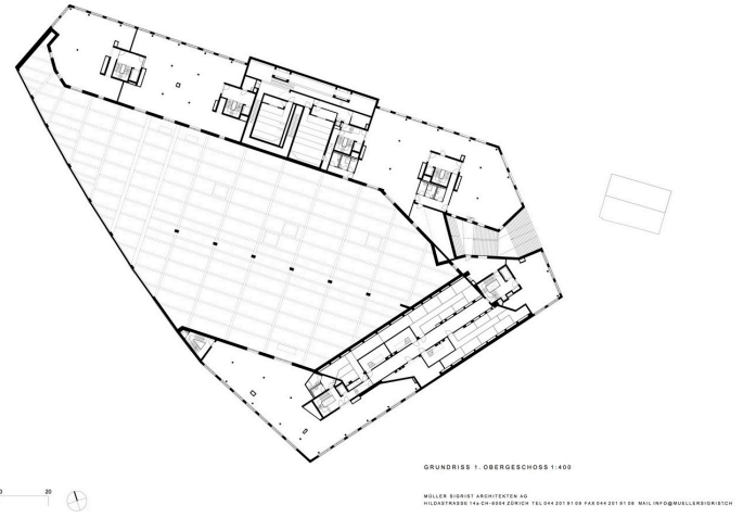
[F39] Planta primera Font: Müller Sigrist Architects
