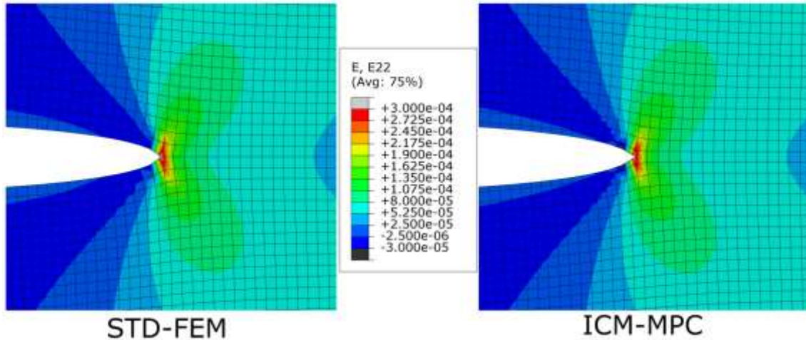
Fig. 3 Comparison of the strain component normal to the crack plane obtained using an explicit crack model (STD-FEM technique) and the ICM-MPC method.
