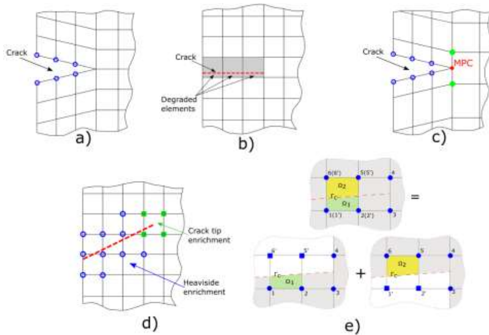
Fig. 1 Schemes of the different numerical modelling techniques analysed in fracture problems. a) Standard FEM (STD-FEM); b) Mechanical property degradation of the elements (MPD); c) Interelemental crack method with MPC (ICM-MPC); d) Extended finite element method (XFEM); e) Phantom node method (PNM).
