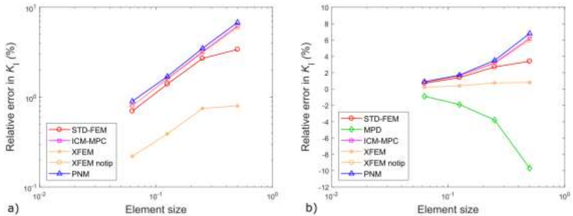
Fig. 9 Convergence analysis for an infinite array of collinear cracks. a) Relative error in K_I (in %) with logarithmic axes; b) Relative error in K_I (in %) with linear vertical axis.
