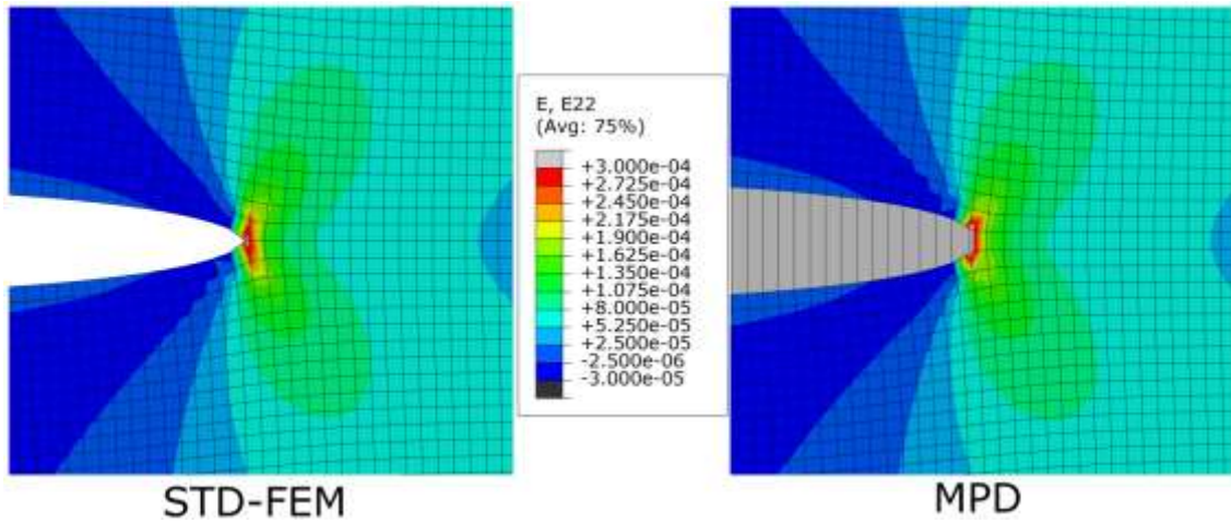
Fig. 2 Comparison of the strain component normal to the crack plane obtained using an explicit crack model (STD-FEM technique) and a reduced stiffness approach (MPD method) for the elements intersected by the crack.
