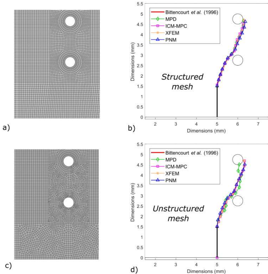
Fig. 14 Crack path numerical predictions for a fracture test reported in Bittencourt et al. 1996 and comparison with the experimental crack path. a) Structured mesh used in the model; b) Results obtained with the structured mesh; c) Unstructured mesh used in the model; d) Results obtained with the unstructured mesh.
