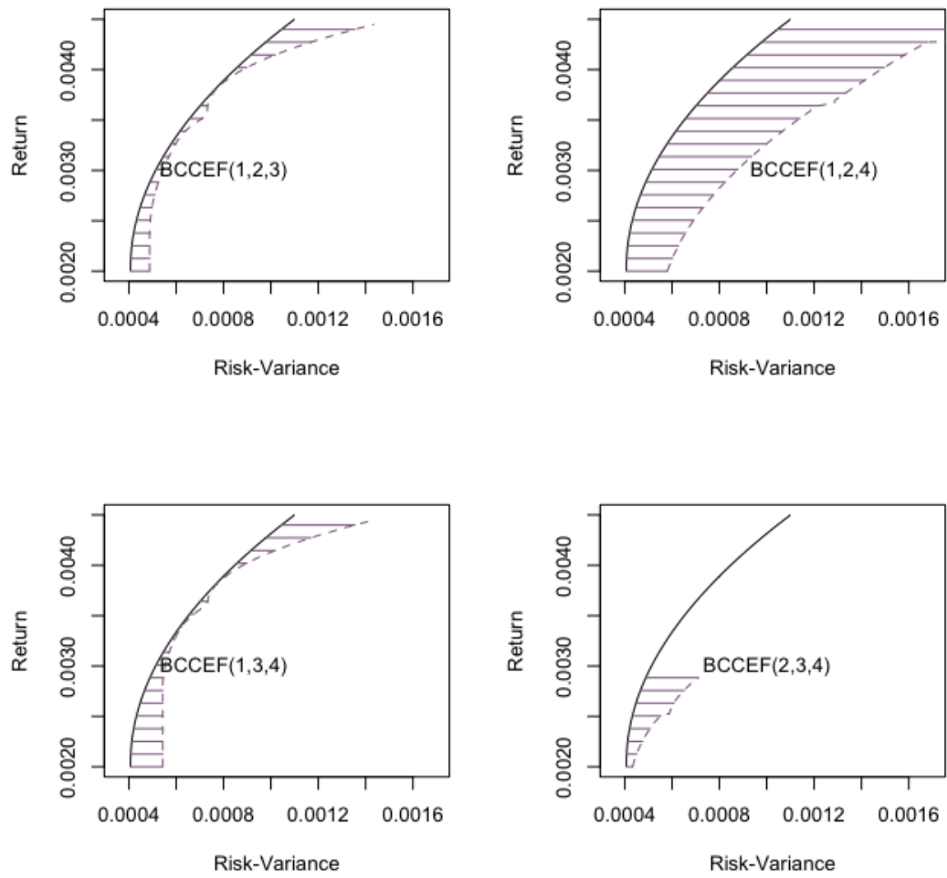
Figure 5. The surrogate similarity measure for different bounded and cardinality constrained frontiers with k = 3 .
