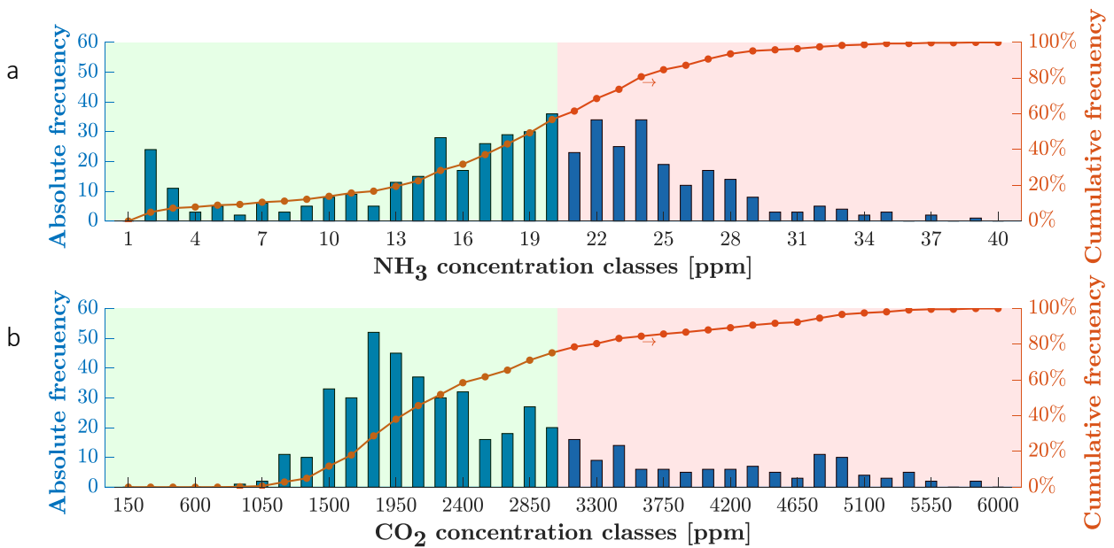
Fig. 4. Absolute and cumulative frequencies of: a) monitored indoor average NH_3 concentration ( \bar{C}_{i,NH_3} ); b) monitored indoor average CO_2 concentration ( \bar{C}_{i,CO_2} ) (arrows indicate the reference axis).
