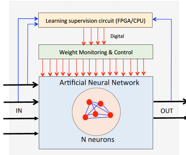
Fig. 36. Schematic description of a neuromorphic processor (after [148]). While two layers of electronics provide control, supervision and reconfigurability, the programmable artificial neural network operates as the core processor.
