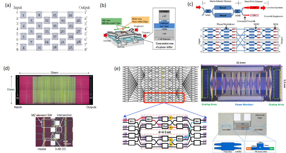
Fig. 35. (a) Layout of a passive 8x8 InP switch fabric (after [140]). (b) Detail of the elementary 2x2 switch cell corresponding to (a). (c) Active 2x2 interferometric InP switch cell combining an MZI and semiconductor optical amplifiers and construction of a 4x4 switch fabric by dilated combination of such cells (after [142]). (d) Photograph and detail of a 2x2 switch cell of a Silicon Photonics 32x32 switch fabric incorporating 1024 MZIs switching cells and thermo-optic phase shifters (after [143]). (e) Layout and chip photograph of a 32x32 switch fabric incorporating 144 MZIs switching cells and carrier injection PIN activated phase shifters. Also shown the basic switch cell unit with push-pull biasing and the 8x8 Benes building block (after [144]).
