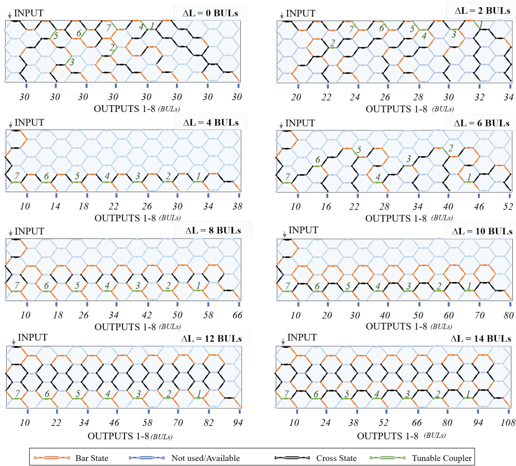
Fig. 19. 1X8 Delay-line array based on discrete optical delay lines: Configuration examples for 0-, 2-, 4-, 6-, 8-, 10-, 12-, and 14-BUL path difference. Each path length is labelled at each output. The color-coded used for each TBU configuration is: Cross State (black), Bar State (Orange), Tunable Coupler (Green).
