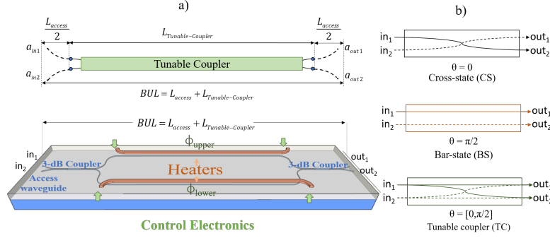
Fig. 13. (a) (Upper) Labelled schematic of a general tunable coupler acting as the basic building block of the mesh. The Basic Unit Length (BUL) is illustrated as the sum of the tunable coupler length and the arc length of the access waveguides. (Lower) Particular case of an integrated balanced MZI-based tunable coupler. (b) Signal flow for the different TBU configuration states.
