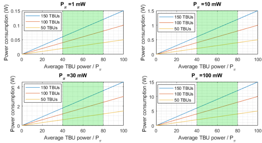
Fig. 29. Overall power consumption for waveguide meshes of 50, 100 and 150 activated TBUs for four different TBU power consumption.
