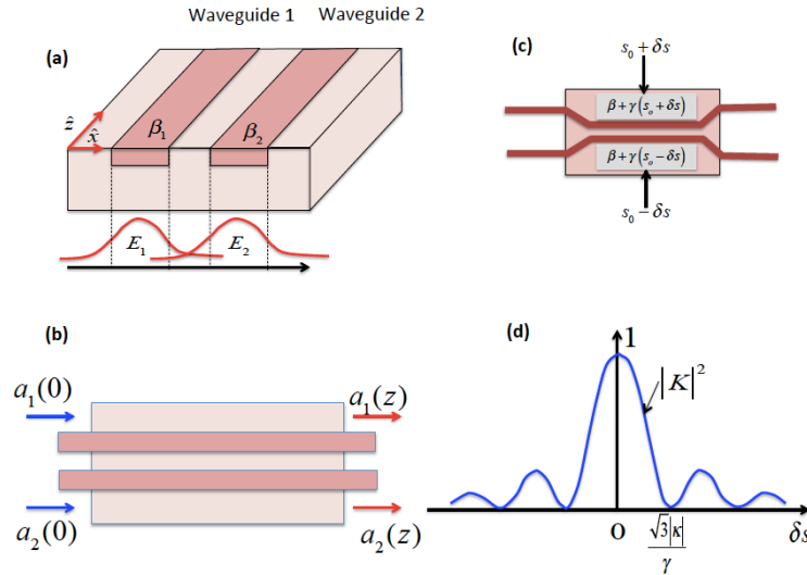
Fig. 5. Schematic (a) cross-section and lateral and (b) top view of a directional coupler. (c) Tunable dual drive directional coupler layout including common mode and differential control signals. (d) Tuning curve for the coupling constant value of a reconfigurable directional coupler versus the differential bias signal.
