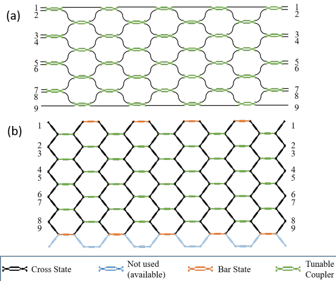
Fig. 32. (a) Rectangular arrangement of a 9x9 interferometer as proposed in [22]. (b) Equivalent implementation using the hexagonal waveguide mesh (after [23]).
