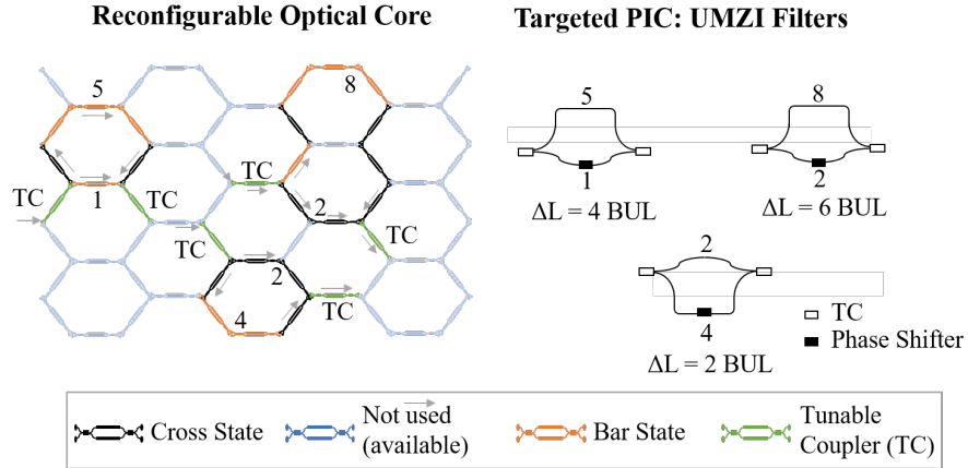
Fig. 17. FIR filter implementations. (Left) hexagonal mesh setting for (Right) three different targeted UMZI Filters. Note the colour code that describes the programming status of each TBU in the mesh.
