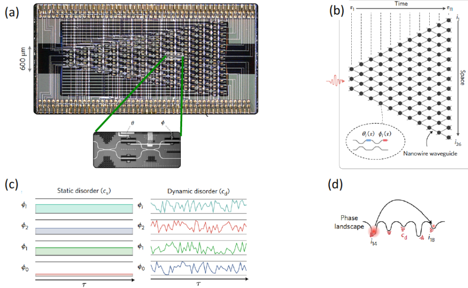
Fig. 34. (a) Silicon programmable processor reported in [15] to simulate discrete-site quantum transport experiments. The inset shows the layout and the internal and external phase shifters of a MZI unit. (b) Layout of the one photon quantum walker circuit implemented by the processor and coordinate system definition. Time ( \tau ) is defined from left to right. Space ( i ) is defined from top to bottom. Dark lines are silicon nanowire waveguides; circles are programmable MZIs. (c) Phase vs time evolution graphs describing the static and dynamic disorders in the programmable circuit. (d) A stuck transport of quantum particles in strong, statically disordered system to external sites can be optimized by introducing dynamic disorder.
