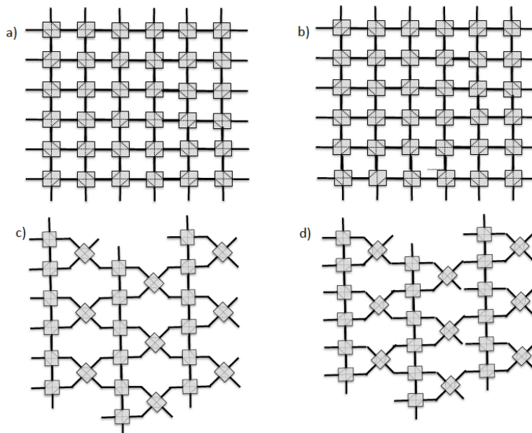
Fig. 23. Physical layouts for the implementation of the 2D gate array in Figure 21. Each square box represents a 2 \times 2 tunable coupling element and a (preceding) phase shifter. The internal broken-dotted lines illustrate the possible physical connections between input and output ports. (a) and (b) show structures where the gates in adjacent columns are rotated by 180^\circ . (c) and (d) show structures where the gates in adjacent columns are rotated by 90^\circ .
