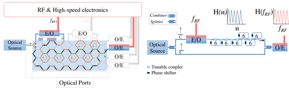
Fig. 40. General-purpose signal processor configuration for RF filtering implementation (left) based on a self-homodyne modulation/detection scheme (right). The optical filter is composed of six cascaded ORRs defined by a cavity length of 6 BULs.
