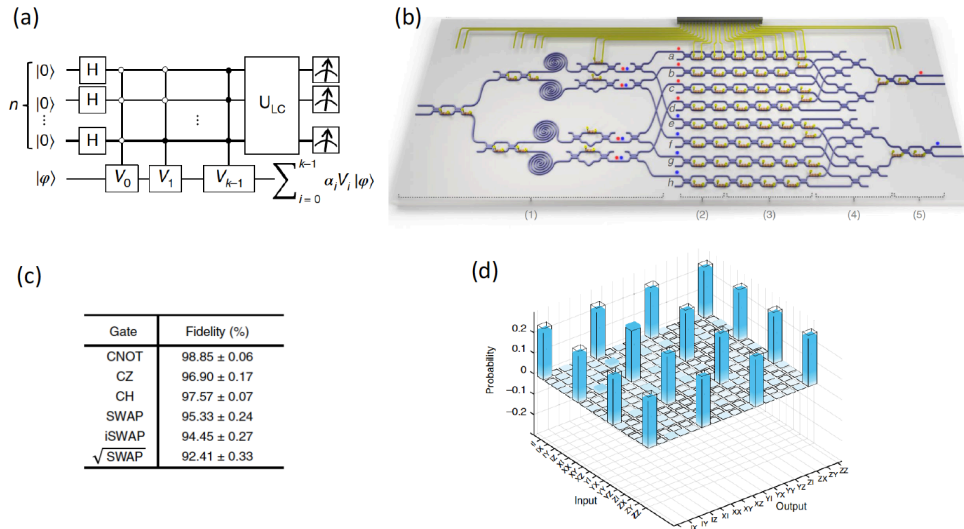
Fig. 33. (a) Layout of a probabilistic implementation of a linear combiner of operators. The linear combination is implemented when all n control qubits are measured to be 0. The success probability is 1/k . (b) Schematic of the silicon photonic chip, which is operated in combination with an external electrical control, laser input and fibre-coupled superconducting detectors. The chip details can be found in the text. (c) Fidelity results for the implementation of several SU(4) gates. (d) Tomography map for the implementation of the SWAP transformation (after [120]),
