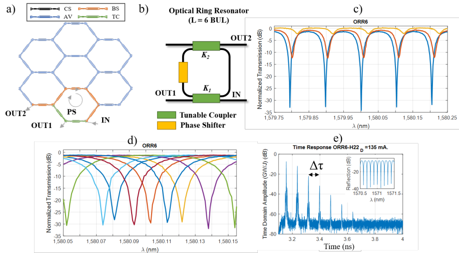
Fig. 27. Experimental results for 6-BUL ring resonator IIR and FIR+IIR filters. (a) Waveguide mesh connection diagram, (b) circuit layout and (c) measured modulus transfer function for a IIR filter for different values of the coupling constants K_1 and K_2 , (d) IIR filter along a full spectral period for different values of the optical ring resonator round-trip phase shift, (e) time response for critical coupling condition.
