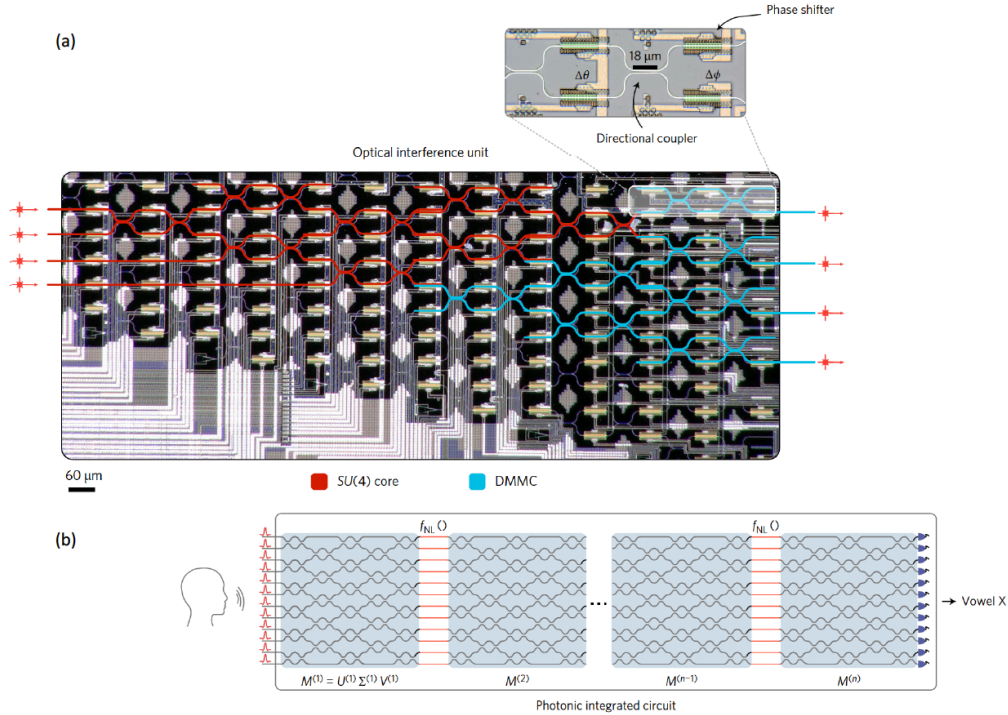
Fig. 38. (a) Optical micrograph illustration of the experimentally demonstrated OIU, which realizes both unitary matrix multiplication (highlighted in red) and diagonal matrix attenuation (highlighted in blue) required for SVD decomposition (after [46]). The inset shows a tunable Mach-Zehnder basic unit (b) Optically implemented artificial neural network assembled for a vowel recognition experiment in [24].
