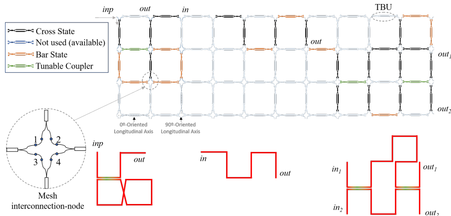
Fig. 14. Basic programming of medium-complex circuits in square waveguide mesh topology: delay line, unbalanced MZI and optical ring resonator.
