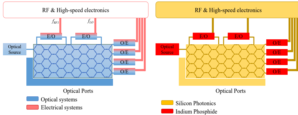
Fig. 39. General-purpose photonic integrated processor architecture and candidate fabrication platforms for each subsystem.
