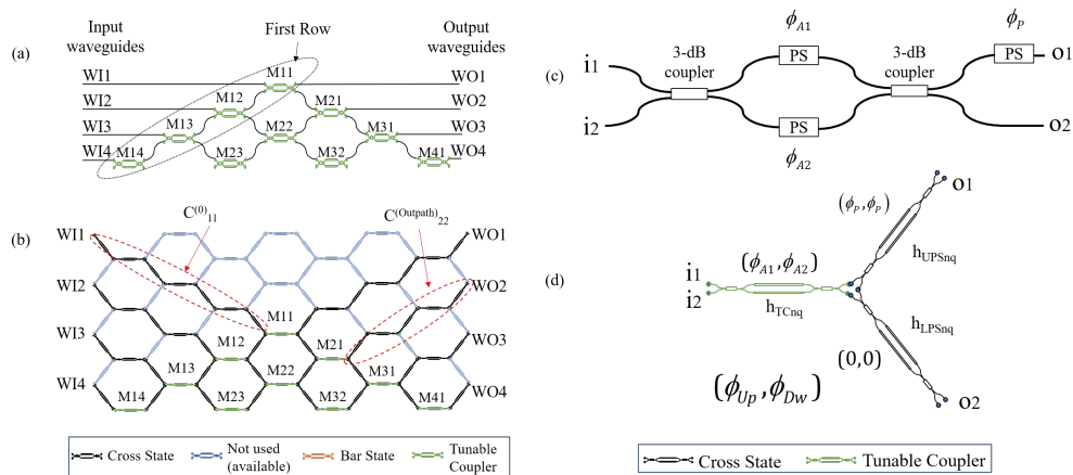
Fig. 20. Universal interferometers: (a) Classical triangular arrangement and (b) hexagonal mesh-based implementation of a 4 x4 interferometer. (c) Beamsplitter for the classical approach and (d) corresponding beamsplitter implementation with 3 TBUs for the hexagonal waveguide Mesh.
