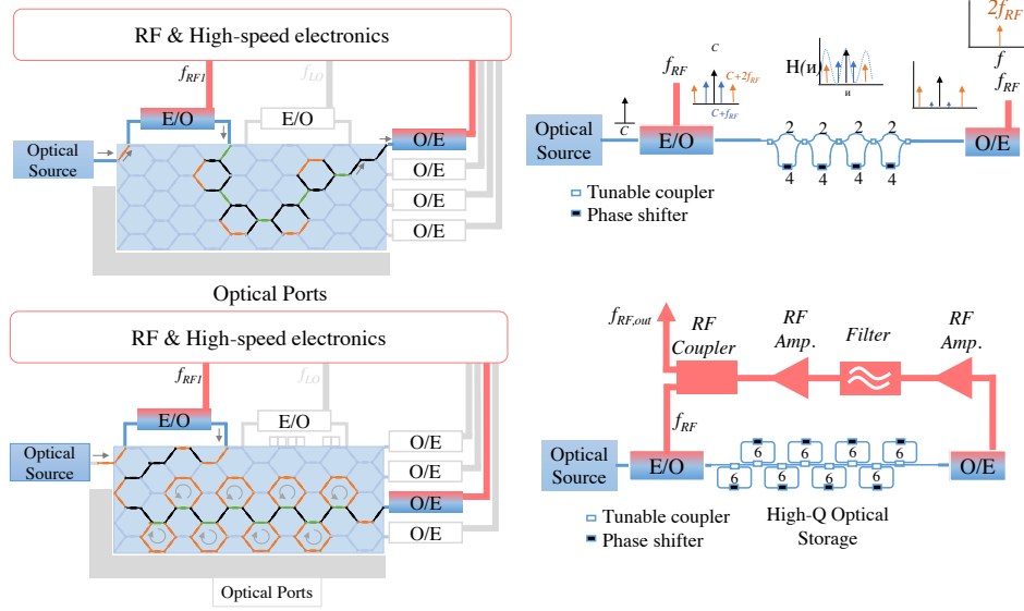
Fig. 41. General-purpose signal processor configuration for microwave and mm-wave tone generation based on (upper) external modulator approach, (bottom) optoelectronic oscillation approach. The right figures illustrate the targeted configuration schemes.
