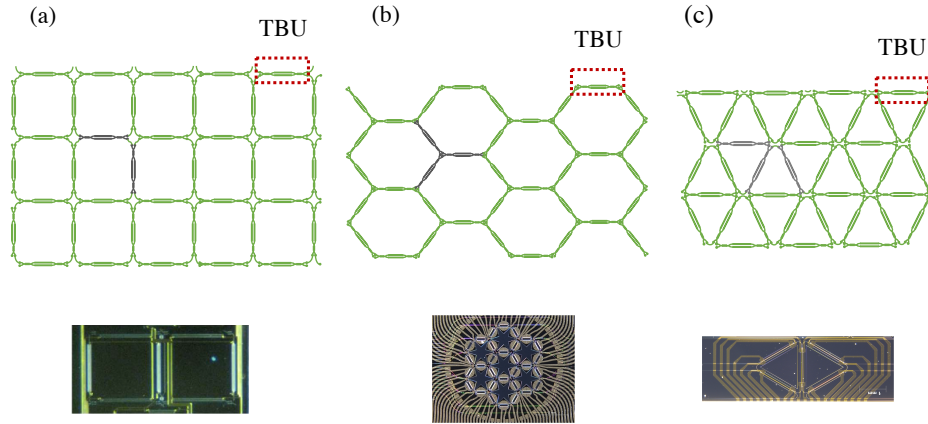
Fig. 12. Different integrated waveguide mesh arrangements: (a) Squared Feedforward/backward and implementation in \text{Si}_3\text{N}_4 [17], (b) Hexagonal Feedforward/backward [20], [31] and implementation in SOI, (c) Triangular Feedforward/backward and implementation in \text{Si}_3\text{N}_4 [18], [64].
