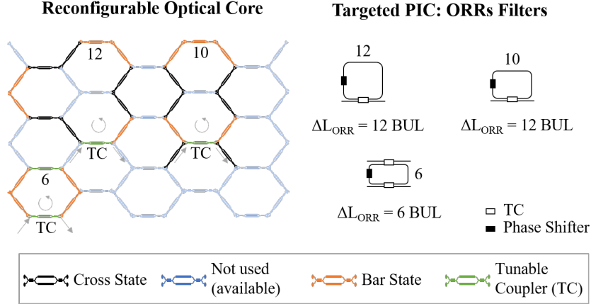
Fig. 18. Single-cavity IIR Filter implementations. (Left) hexagonal mesh setting for (right) three different targeted ORR filters. Note the colour code that describes the programming status of each TBU in the mesh.
