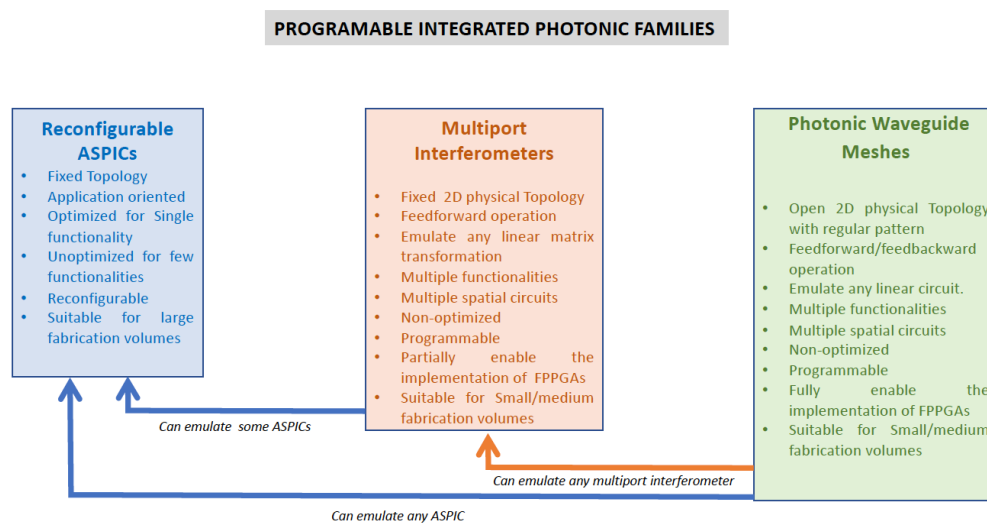
Fig. 1. Classification and features of the main Programmable Integrated Photonic families.
