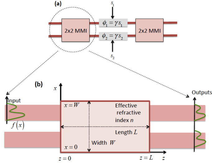
Fig. 6. (a) Tunable 3-dB MZI coupler, (b) layout of the 2x2 3-dB Multimode Interference (MMI) coupler used to embed the balanced interferometer.
