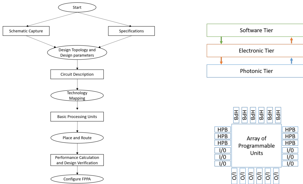
Fig. 25. Left: main steps involved in the design Flow of a FPPGA device. Right: FPPGA soft and hard tiers and expanded layout including peripheral high-performance blocks.
