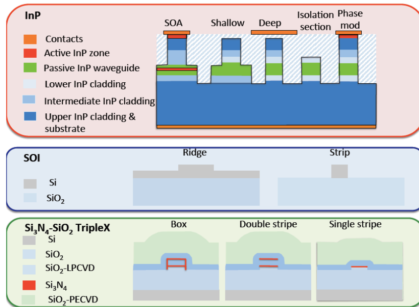
Fig. 2. Waveguide structures for the InP (upper row) SOI (intermediate row) and Si 3 N 4 -SiO 2 (lower row) platforms.
