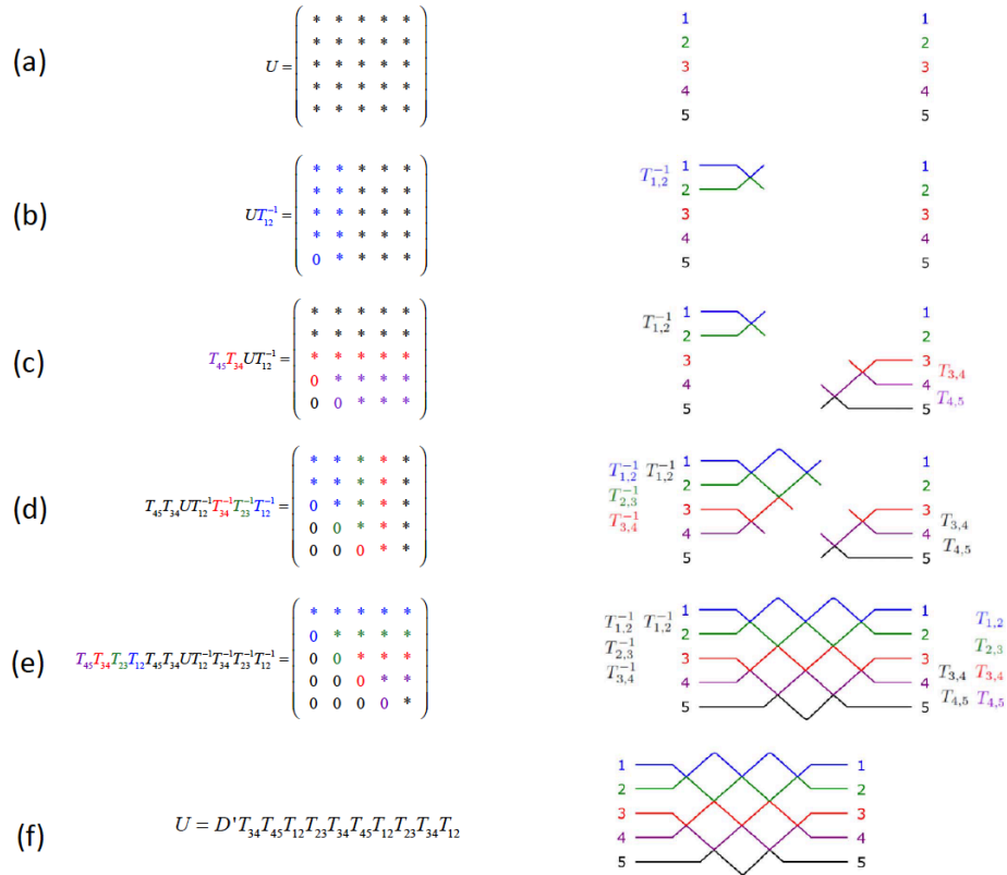
Fig.10. Illustration of the algorithm for programming a universal multiport interferometer for U(5) interferometer (After [22]). The left-hand side presents the decomposition procedure, and the right-hand side shows how the decomposition for building up the corresponding interferometer. (a) The starting point is any random unitary matrix U(5) and a blank interferometer. (b)-(e) Successive stages of the implementation algorithm. (f) Final expression for U(5) in terms of a cascade of U(2) interferometers and a diagonal matrix.
