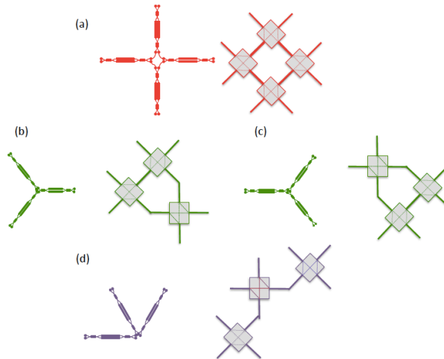
Fig. 24. Identification between the fundamental unit blocks employed to construct integrated waveguide meshes and the main physical layouts for 2D gate arrays shown in Fig. 23.
