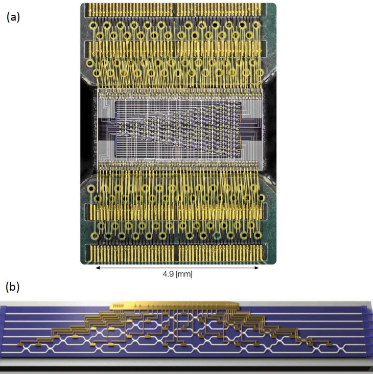
Fig. 31. (a) Optical micrograph of 26-mode, 88-MZI Silicon photonics programmable core (after [59]). (b) Germanium-doped glass six-mode, 15-MZI Silica on Silicon programmable core (after [13]).
