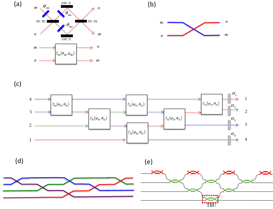
Fig. 9. (a) Bulk optics implementation of a tunable beam splitter (After [21]). (b) Symbol representation of the beam splitter layout. (c) Triangular decomposition implementing a general U(4) 4x4 unitary transformation and layout (d). Colours represent the propagation of a given input port. (e) U(4) layout of Figure 8(d) and its implementation using MZI based TBUs. TBUs in red colour operate as phase shifters.
