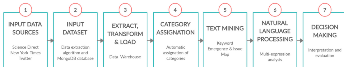
Figure 1. Steps of the system implemented to detect future signals.
