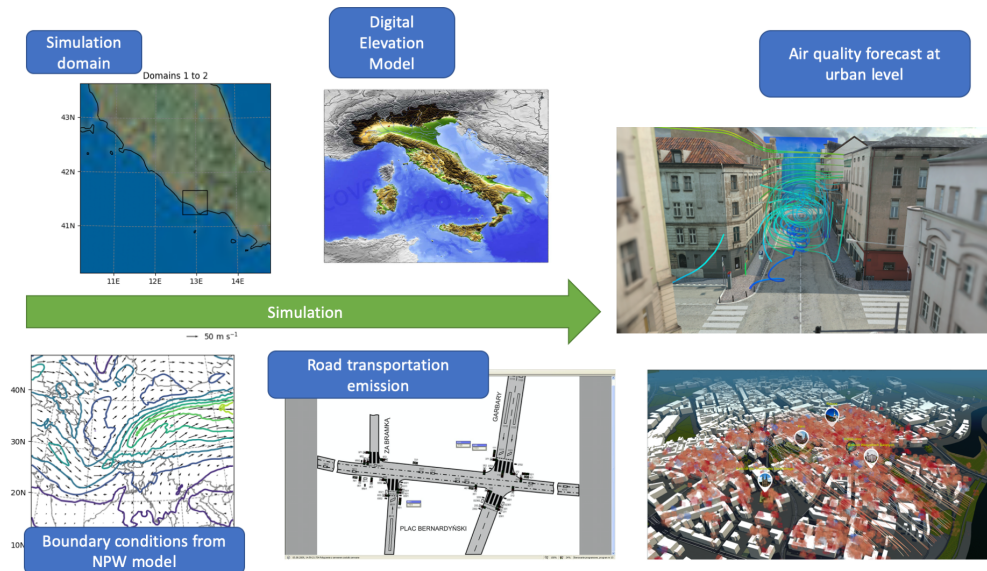
Figure 7: High level representation of the UrbanAir application.
