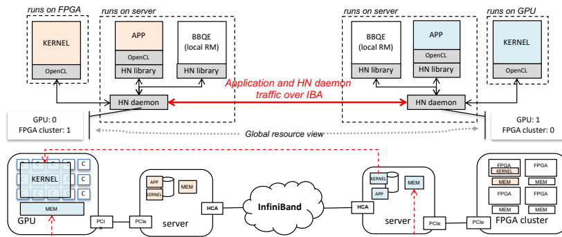
Figure 2: Low-level runtime architecture.
