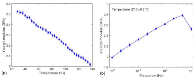
Fig. 9. Young's modulus variation for the 3D PC mPOF as a function of temperature (a) and strain cycle frequency (b). Error bars show mean deviation.
