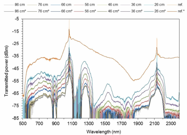
Fig. 6. Transmission spectra for different lengths of the same piece of 3D PC mPOF used for cut-back attenuation calculations. Reference spectrum (marked "ref.") comes from the supercontinuum light source attached directly to OSA. In order to reduce noise, moving averages (darker lines, data series marked with *) have been plotted over original spectra (lighter lines). In this paper, moving averages for each spectral point have been calculated using 5 neighbors to its left and right, resulting in 11 spectral points being averaged over.
