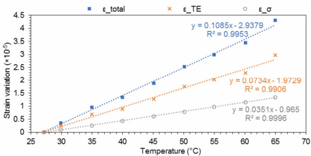
Fig. 10. Strain variation of the 3D PC mPOF ( \epsilon_{total} ) as a function of temperature. It was split into strain due to thermal expansion ( \epsilon_{TE} ) and different response to stress caused by tensile load of 0.01 N, coming from dependence of Young's modulus on temperature ( \epsilon_{\sigma} ). See (1)-(3) for details.
