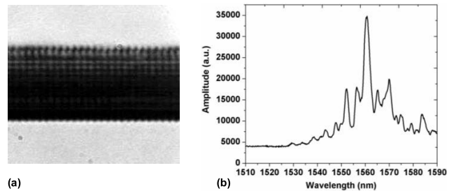
Fig. 13. (a) Microscopic image (side view) of the FBG inscribed in 3D PC mPOF by femtosecond laser (FBG2). (b) Reflection spectrum (4 th order) of FBG2.
