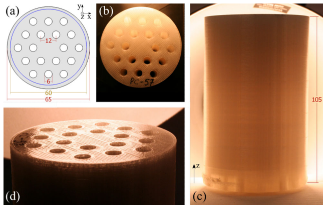
Fig. 2. (a) Top view of the preform design. The blue ring shows the machined down diameter. (b) Top view of the printed preform (illuminated from the top edge). (c) Side view of the printed preform (illuminated from behind). (d) View of the top surface of the printed preform. All dimensions in mm.
