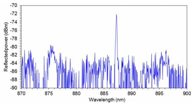
Fig. 15. Reflection spectrum of a 248nm KrF laser-inscribed FBG in the 3D PC mPOF.
