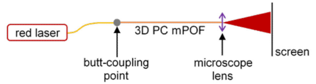
Fig. 4. Schematic showing the experimental setup used for checking core guidance (fiber length = 38.1 mm). The image observed on the screen is shown in Fig. 3(c).
