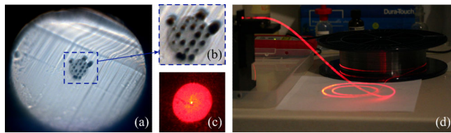
Fig. 3. (a) View of a cleaved fiber facet (blade temperature = 75°C; fiber outer diameter = 170 \mu\text{m} , fiber core diameter = 8 \mu\text{m} ). (b) Magnified view of the fiber core. (c) Image of a fiber end projected on screen (fiber length of 38.1 mm) with clear core guidance. See Fig. 4 for the experimental setup. (d) Photograph of butt-coupling to the fiber on spool.
