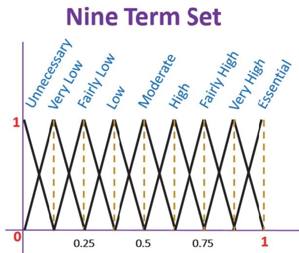
Fig. 6. Linguistic labels
