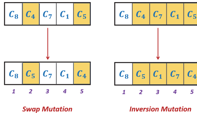
Fig. 11. Mutation Operators
