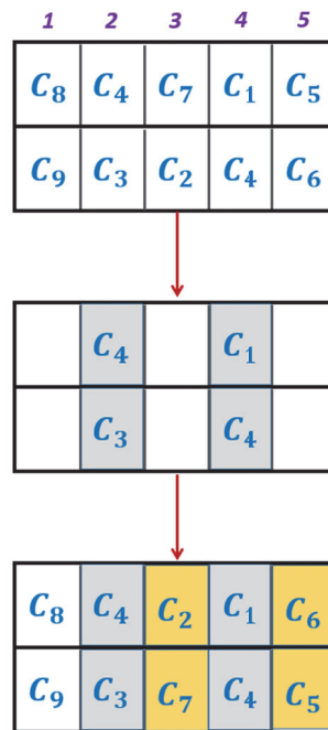
Fig. 10. Permutation crossover
