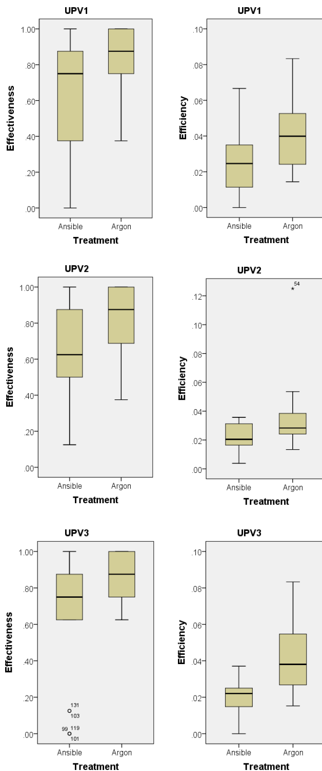
FIGURE 5. Boxplots for treatment effectiveness and treatment efficiency.
