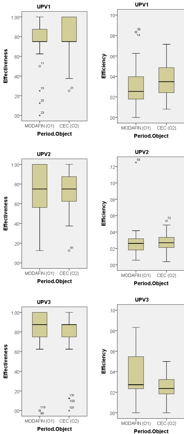
FIGURE 7. Boxplots for period effectiveness and period efficiency.
