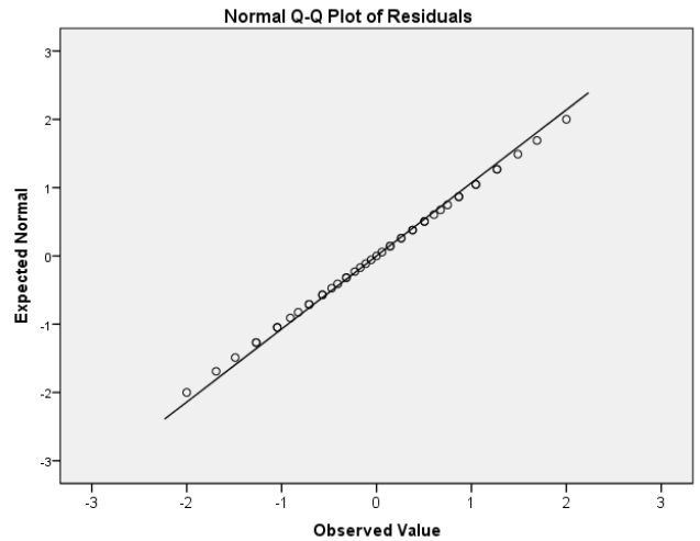
FIGURE 9. Normal probability plot of residuals (Effectiveness).
