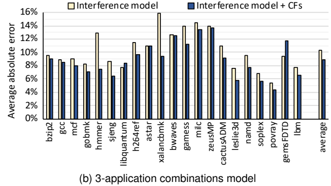
Fig. 4. Per-application average absolute error for the two- and three-application models without and with correction factors.
