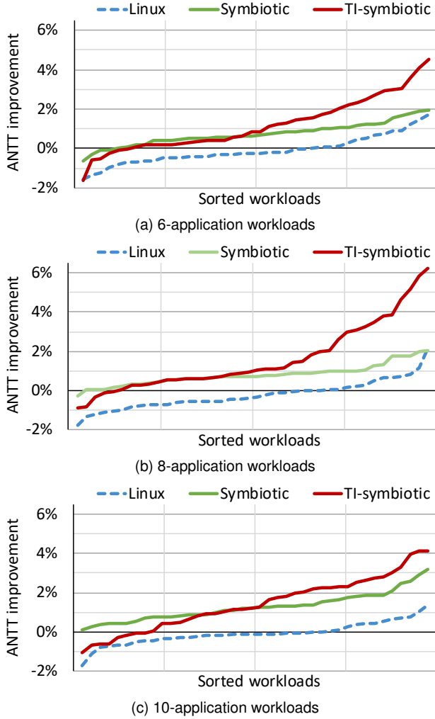
Fig. 6. ANTT improvement for the TI-symbiotic, symbiotic and Linux schedulers relative to random scheduling.
