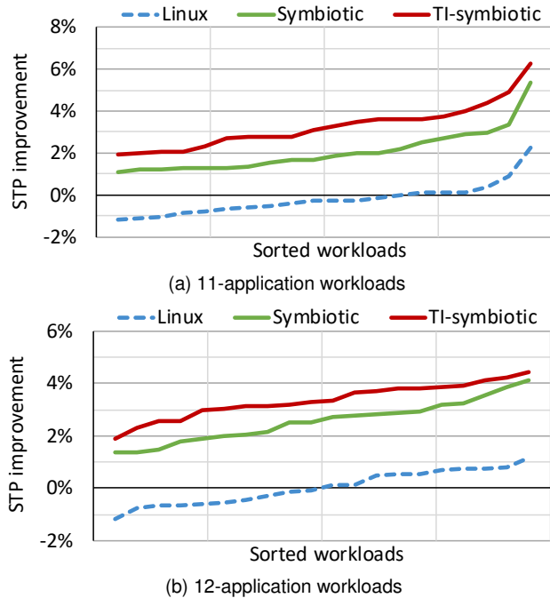
Fig. 10. STP improvement for the TI-symbiotic, symbiotic and Linux schedulers relative to random scheduling running large workloads on 5 cores.
