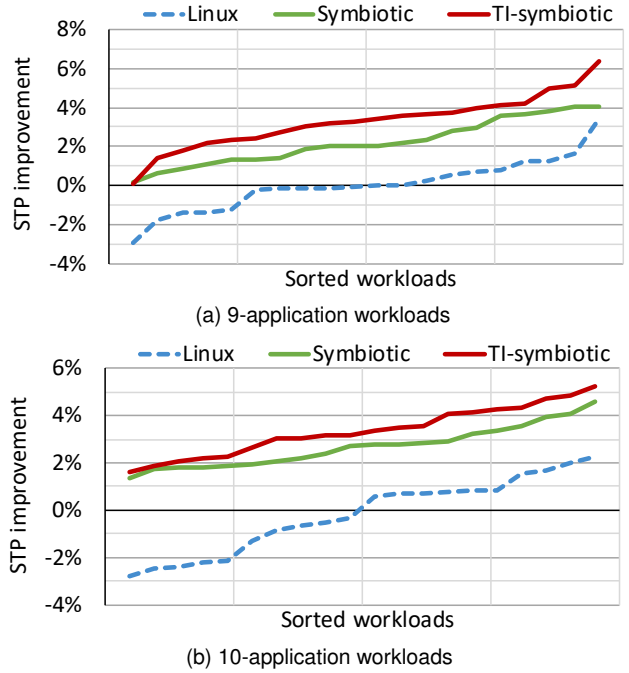
Fig. 9. STP improvement for the TI-symbiotic, symbiotic and Linux schedulers relative to random scheduling running large workloads on 4 cores.
