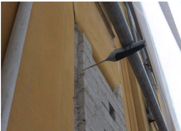
Fig. 17: The thermofluximeter probe, external view
