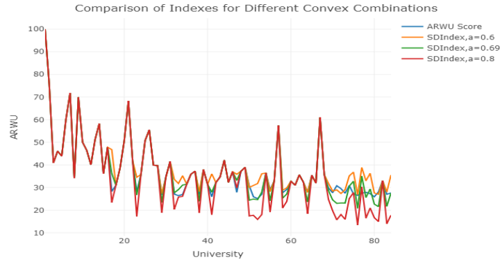
Figure 5: Representation of the error committed by three different values of \alpha = a .
