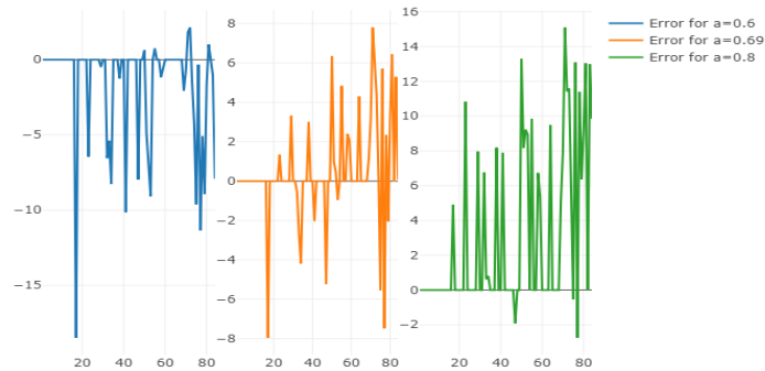
Figure 5: Representation of the error committed by three different values of \alpha = a .
