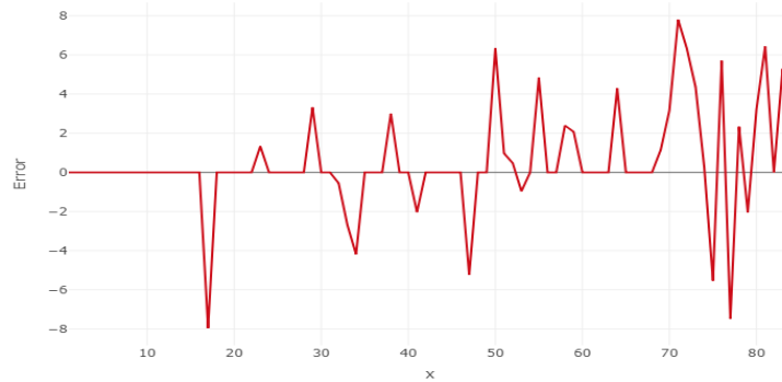
Figure 7: Representation of the error committed by the best choice of convex combination \alpha = 0.69 .
