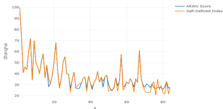
Figure 6: Representation of the best solution together with the original values of the ARWU score ( \alpha = 0.69 ).
