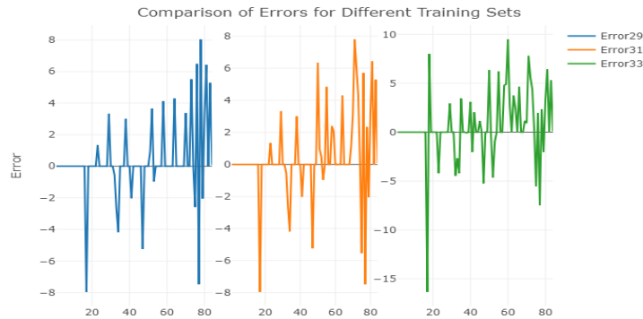
Figure 3: Representation of the error for three different training sets.
