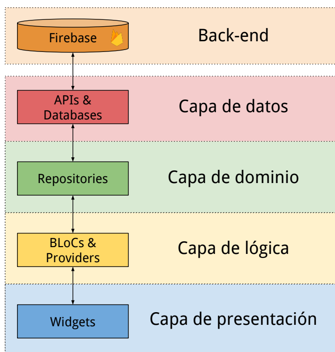
Figura 4.5: Diagrama de Diagrama Clean Architecture
