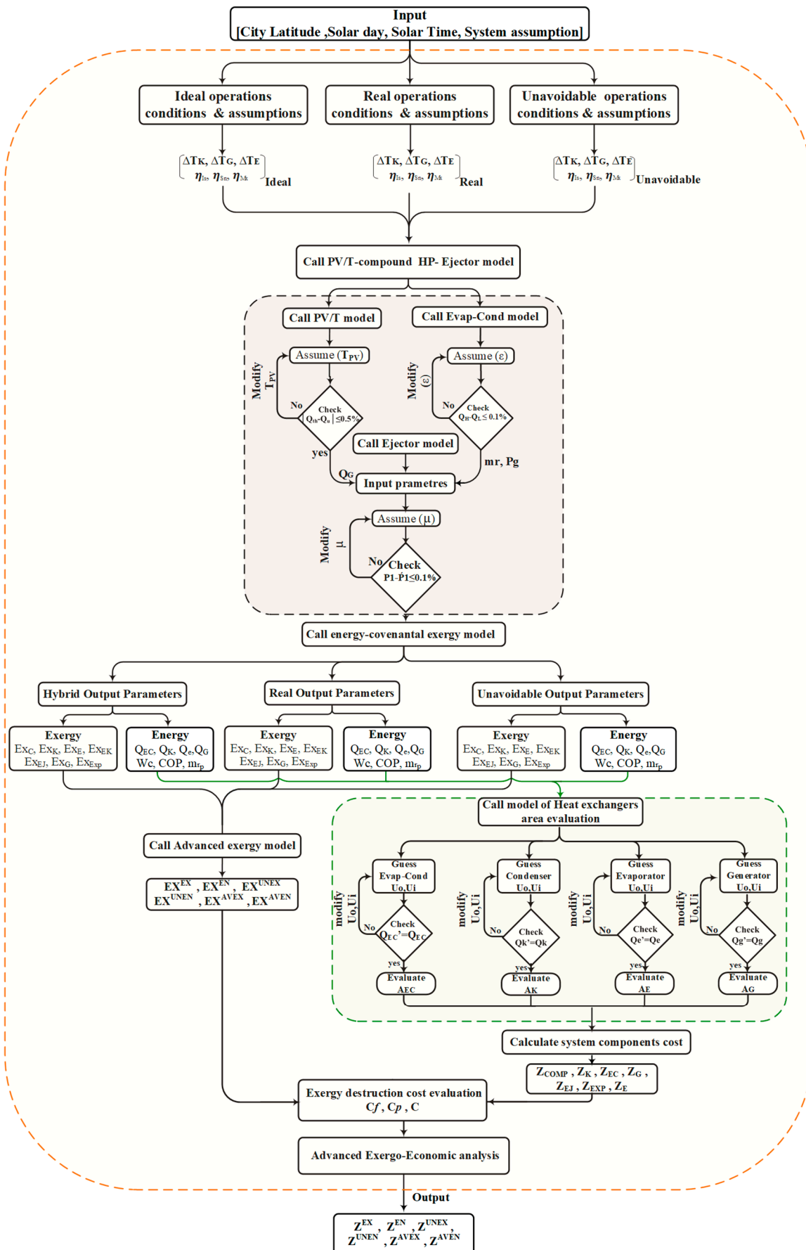
Figure 2. Flow diagram for the system methodology.
