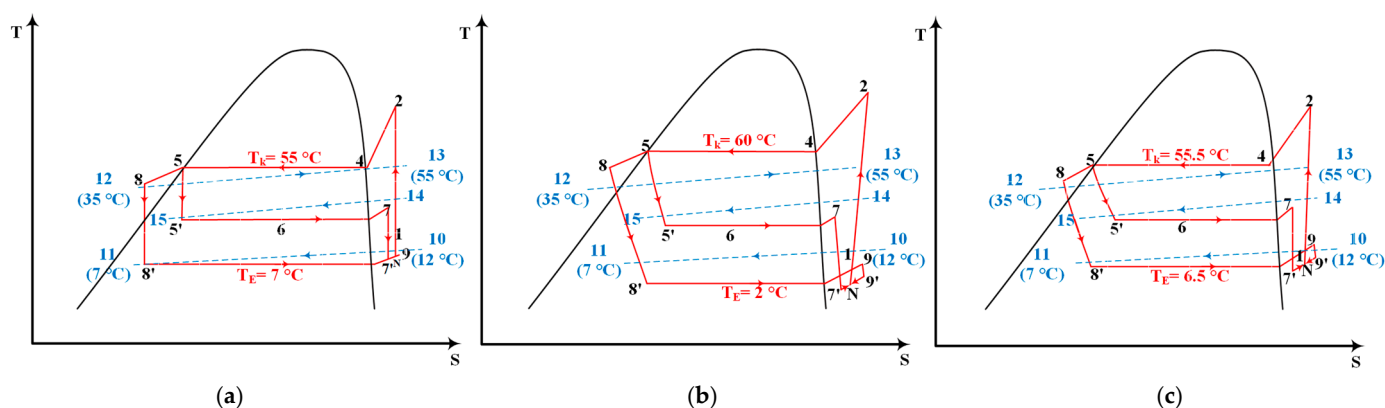
Figure 3. T-s diagram of the investigated system under different conditions: (a) ideal, (b) real, and (c) unavoidable.
