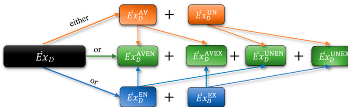
Figure 4. Exergy destruction splitting within a component for advanced exergy analysis.
