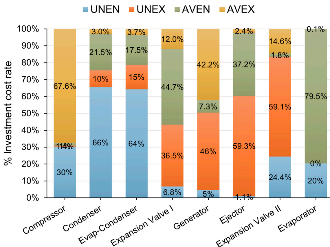
Figure 13. Percentage of components cost rate.
