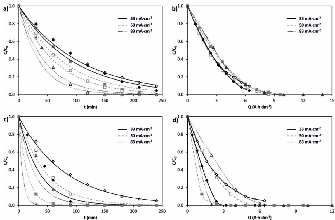
Figure 3. Evolution of the relative concentration of ATL as a function of time ( t ) and applied charge per unit volume ( Q ) for the undivided reactor (a and b) and the divided reactor (c and d) at different current densities. Solid points represent BDD electrode and empty points the ceramic electrode.
