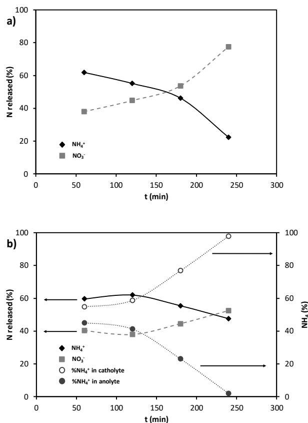
Figure 7. Evolution of the percentage of total nitrogen released in the form of \text{NH}_4^+ or \text{NO}_3^- as a function of time for (a) undivided and (b) divided reactor at 50 \text{ mA}\cdot\text{cm}^{-2} using BDD electrode.
