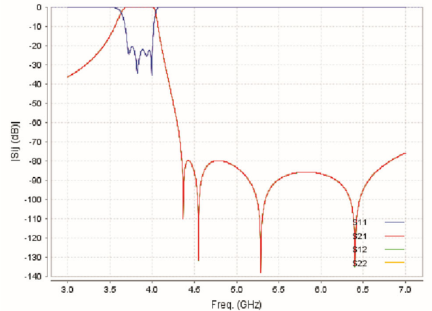
Fig. 5. Four pole filter with both inductive and capacitive inter resonator couplings.
