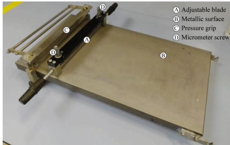
Figure 3. Coating equipment.
