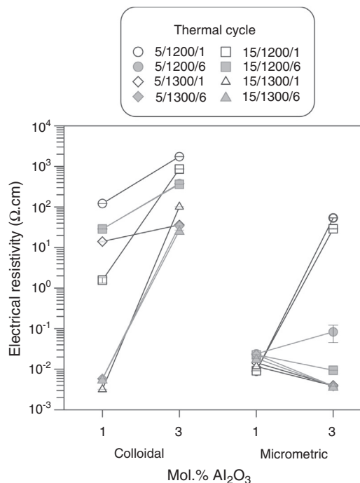
Fig. 8 – Specimens' electrical resistivity as a function of the percentage of alumina (colloidal or micrometric) and thermal cycle parameters (heating rate/ T_{\text{max}} /soaking time).
