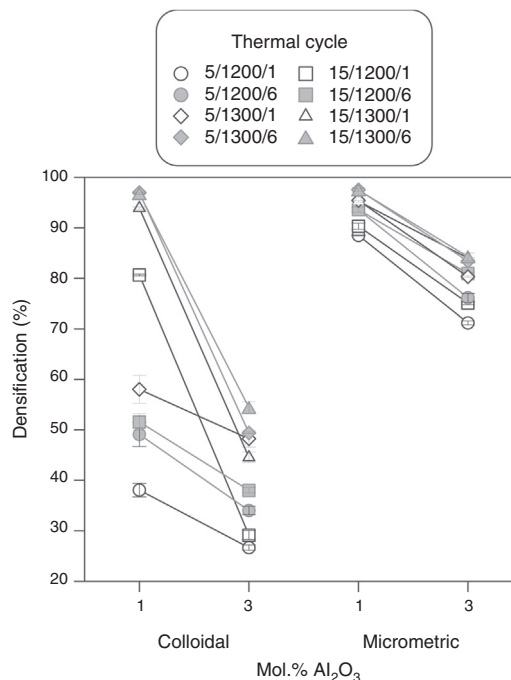
Fig. 7 – Specimen' densification as a function of the percentage of alumina (colloidal or micrometric) and thermal cycle parameters (heating rate/ T_{\text{max}} /soaking time).
