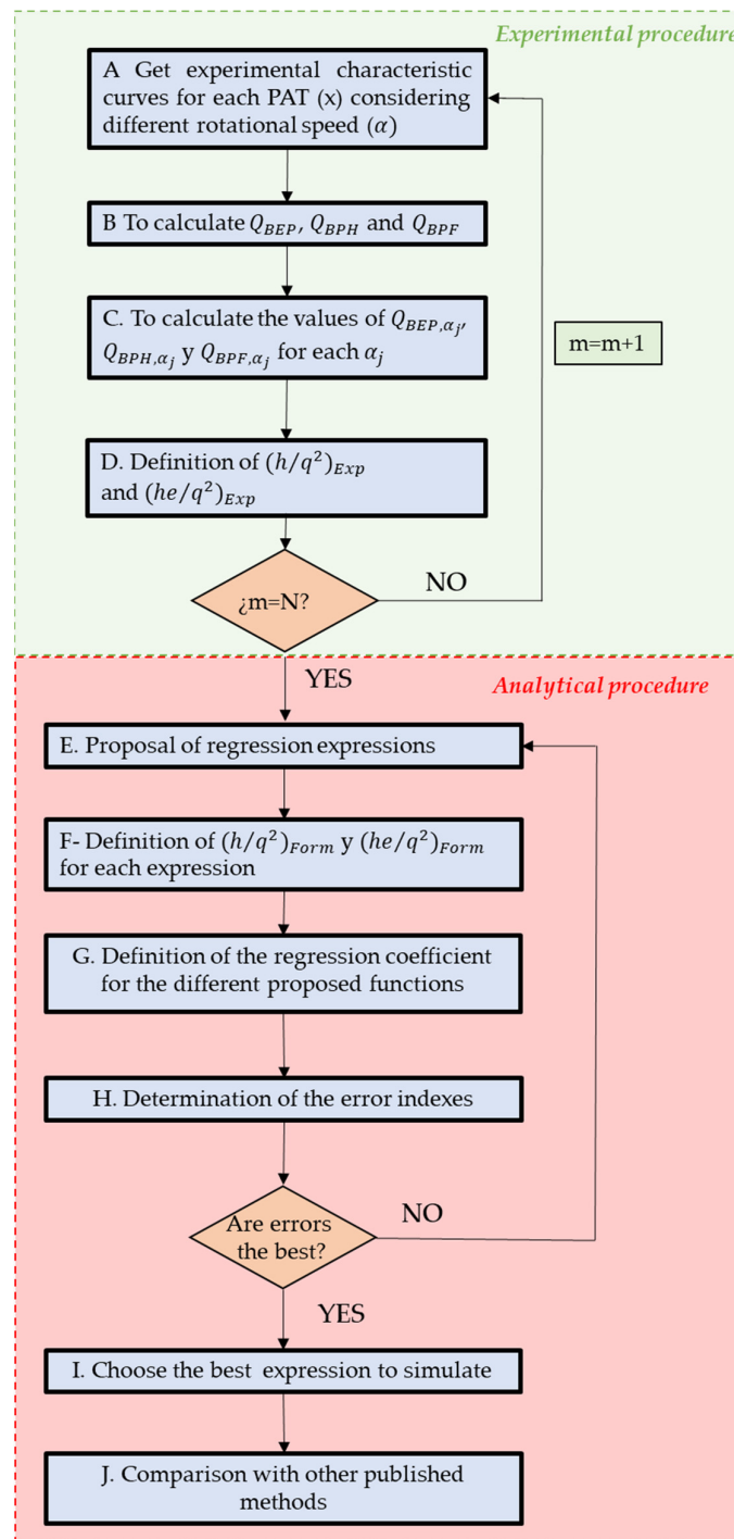
Figure 2. The methodology proposed to reach the expressions.
