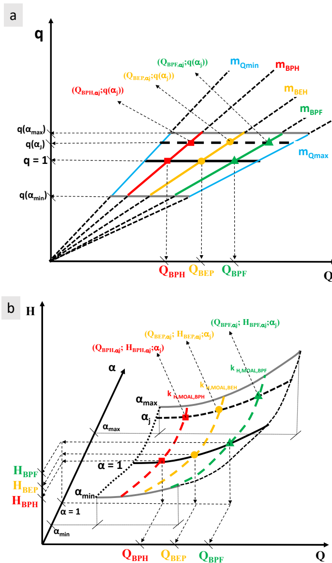
Figure 1. (a) m coefficient; (b) VOS zone.
