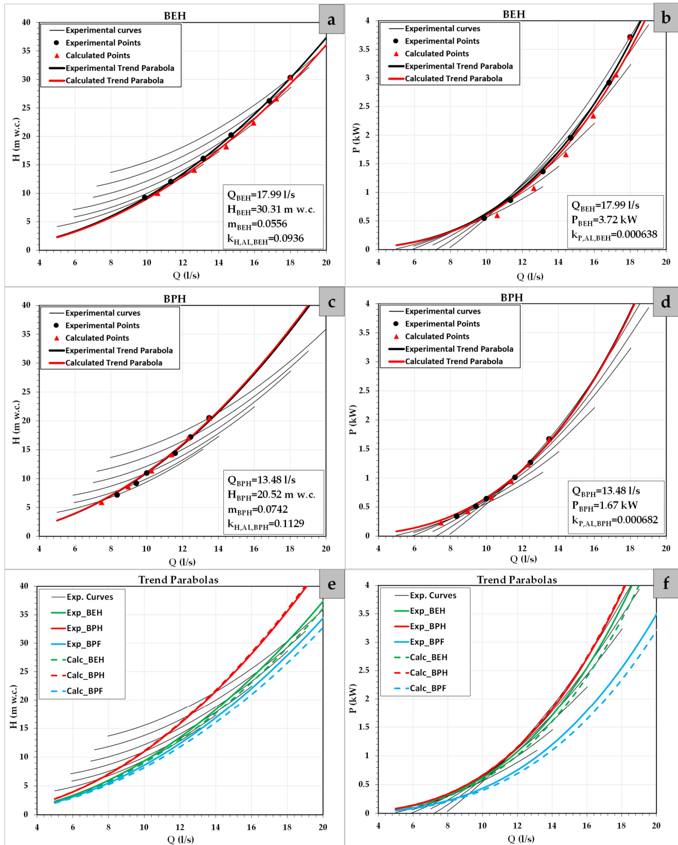
Figure 5. (a) H-Q for BEH; (b) P-Q for BEH; (c) H-Q for BPH; (d) P-Q for BPH; (e) H-Q for BEH, BPH and BPF; (f) P-Q for BEH, BPH and BPF.
