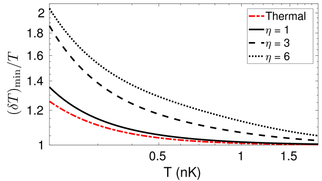
FIG. 1. (color online) (black) Optimal relative error (\delta T)_{\min} / T ( \nu = 1 ) as a function of the temperature of the BEC in a logarithmic scale. Specifically, we work with impurities of Yb in a sea of ultra-cold K. The temperature range for the BEC is 200 \text{ pK} \leq T \leq 2 \text{ nK} . The trapping frequency of the gas (with N = 5000 atoms) was set to \omega_B = 2\pi \times 100 \text{ Hz} , while \Omega = 2\pi \times 10 \text{ Hz} ( g_{rmB} = 3 \times 10^{-39} \text{ Jm} ). Different probe-sample coupling ratios \eta = g_{IB}/g_B were considered, namely (solid) \eta = 1 , (dashed) \eta = 3 , and (dotted) \eta = 6 . For comparison, we also depicted the relative error of a fully thermalized impurity (i.e., \eta \rightarrow 0 ) (dot-dashed red). Note that, for \eta = 1 , the relative error can be kept below \sim 14\% from only \nu \sim 100 measurements. This is quantitatively close to state-of-the-art destructive experimental techniques. See text for discussion.
