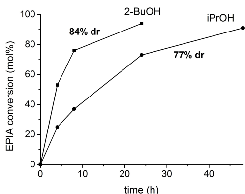
Figure 5. MPV reduction of epiandrosterone (EPIA) to androstane-diols using i PrOH and 2-BuOH. The obtained diastereoselectivity ( dr ) to \alpha -EPIAdiol is indicated. dr was calculated by ^1\text{H} NMR of the filtrate at the end of the reaction (see the Supporting Information). Reaction conditions: 23 mg of EPIA (0.08 mmol), alcohol (ca. 16 equiv) and Zr catalyst (5 mg, ca. 18 mol% Zr), 393 K.
