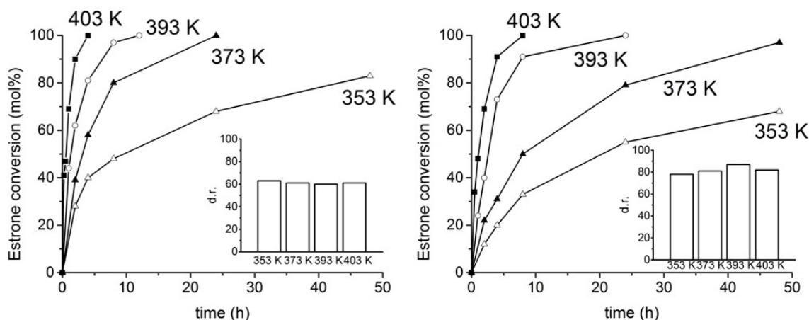
Figure 2. Time-conversion plots of MPV reduction of estrone by using MOF-808 with isopropanol (left) or butan-2-ol (right) over the temperature range 353–403 K. In each plot, the inset shows the diastereomeric ratio of the reaction, dr ( \alpha -E2: \beta -E2).
