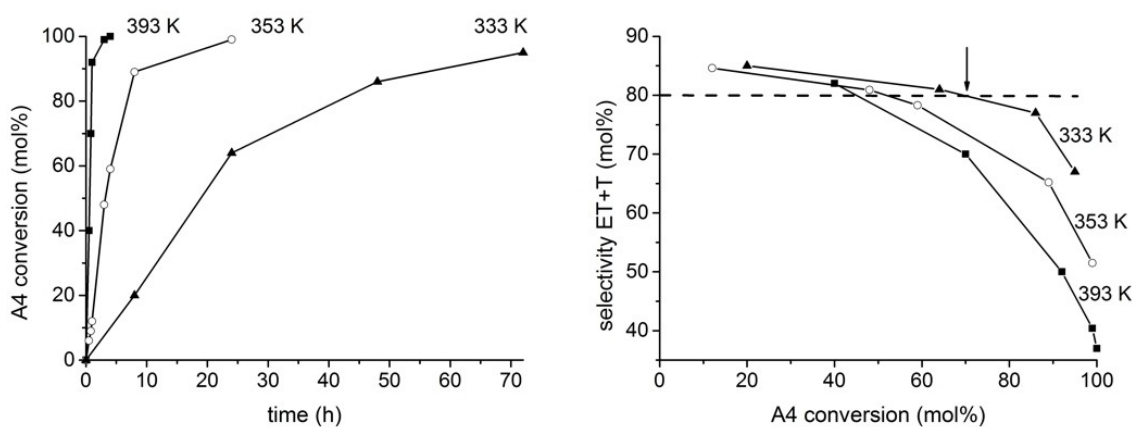
Figure 7. Left: A4 conversion over MOF-808 in 2-BuOH at the indicated temperature. Right: Selectivity to monohydroxylated products, ET+T, as a function of the A4 conversion and temperature.
