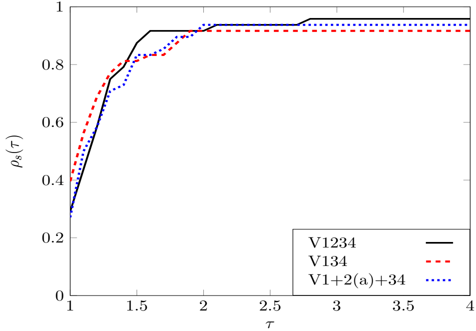
Figure 8: Impact of the parity inequalities: Performance profile
