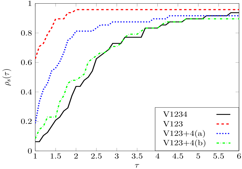
Figure 9: Impact of the max-distance inequalities: Performance profile
