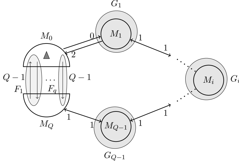
Figure 5: Disaggregate K-C_{02} inequalities for the DC-CEARP
