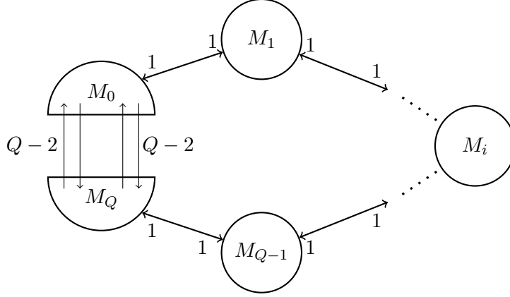
Figure 2: Standard K-C basic structure.
