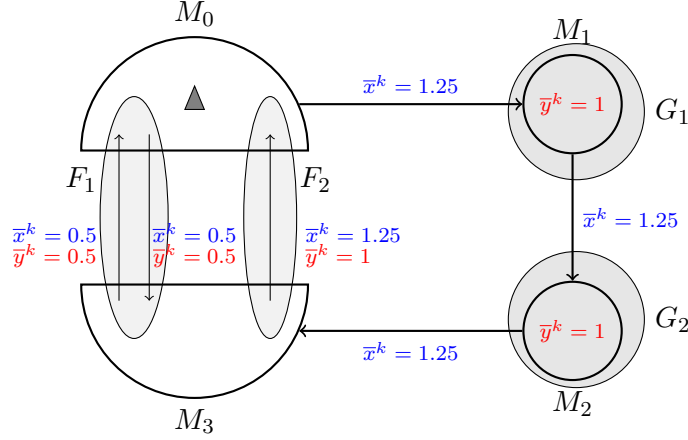
Figure 4: A fractional solution for vehicle k not cut off by a disaggregate K-C inequality
