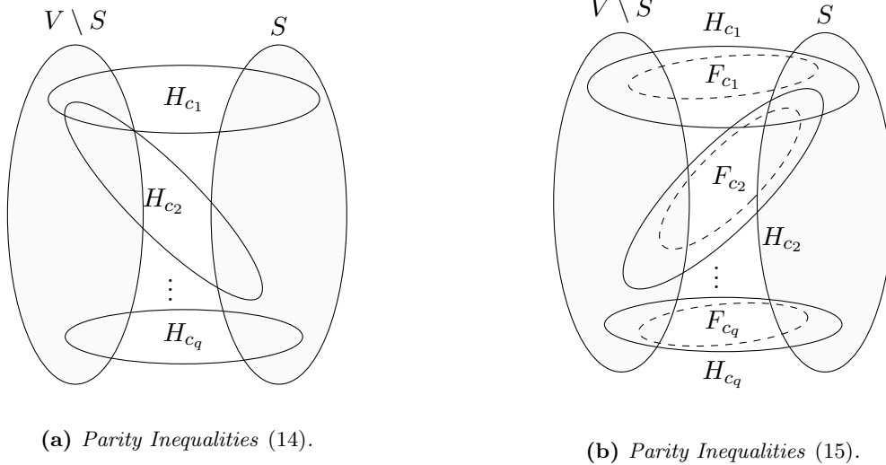
Figure 1: Structure of the parity inequalities for the DC-CEARP
