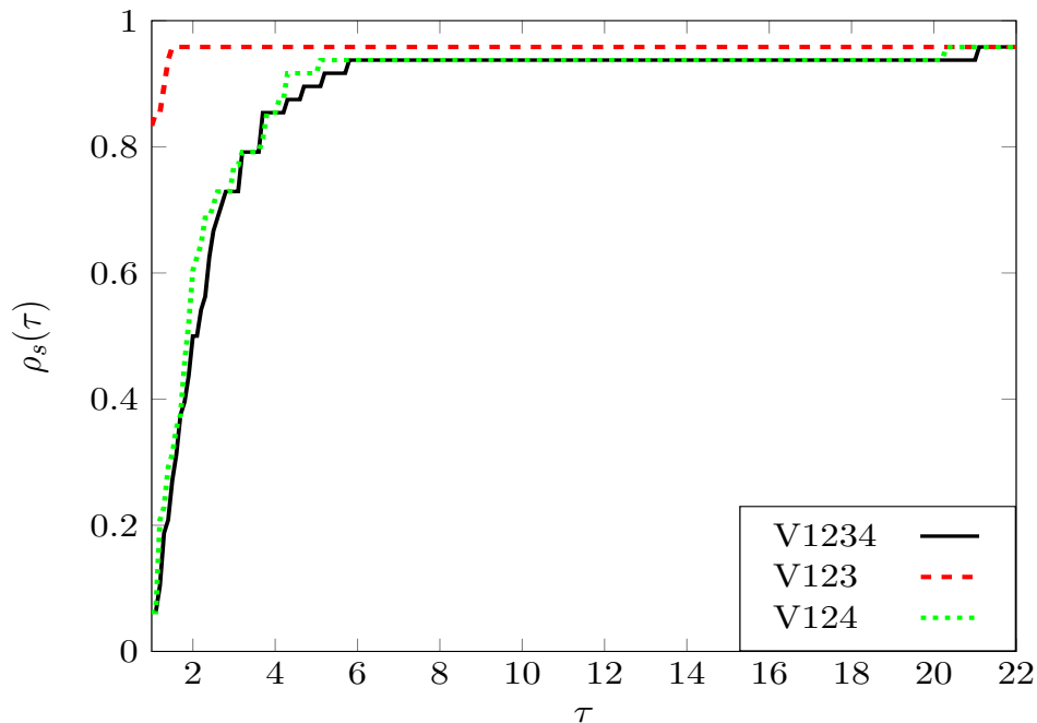
Figure 10: Impact of the K - C , K - C_{02} and Path-Bridge inequalities: Performance profile
