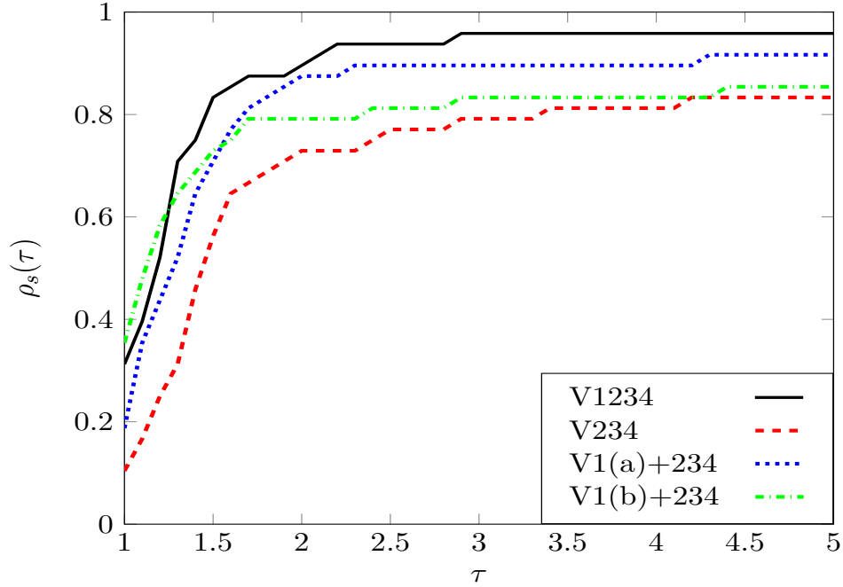
Figure 7: Impact of the connectivity inequalities: Performance profile
