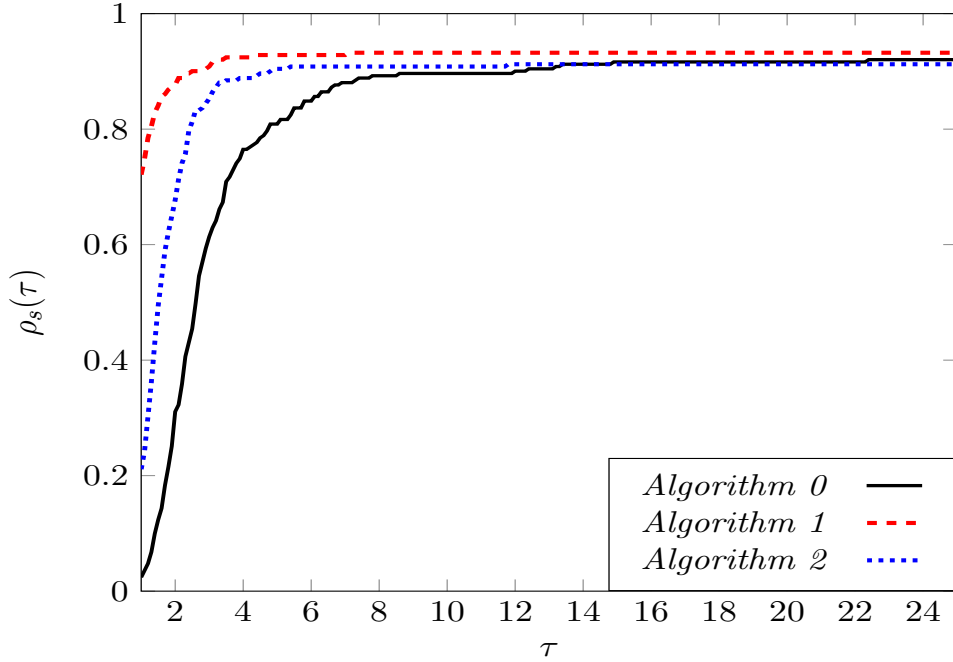
Figure 11: Performance profile
