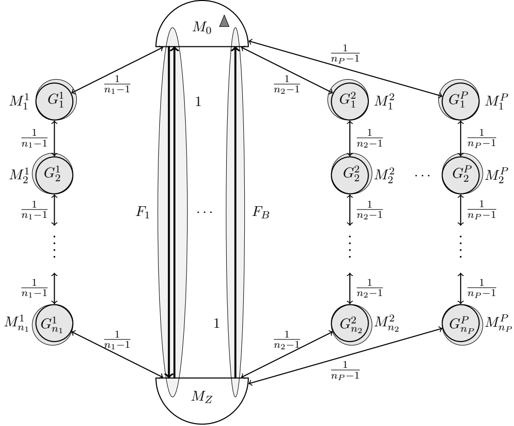
Figure 6: Standard Path-Bridge for the DC-CEARP
