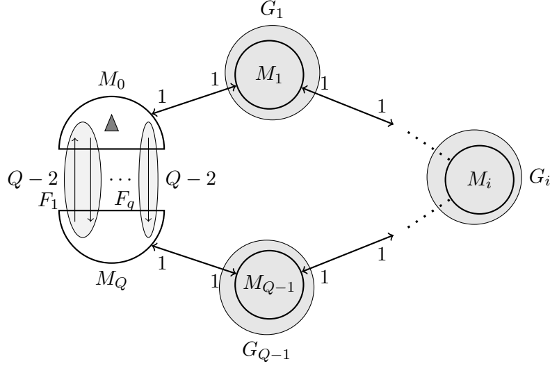
Figure 3: Standard disaggregate K - C inequality for the DC-CEARP. Depot is represented by a triangle
