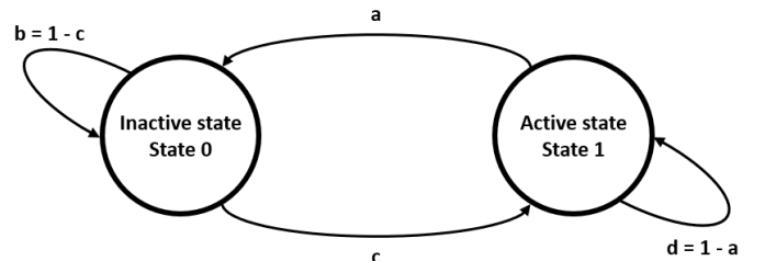
Figure 10: Two-state activity model for one speaker [55].
