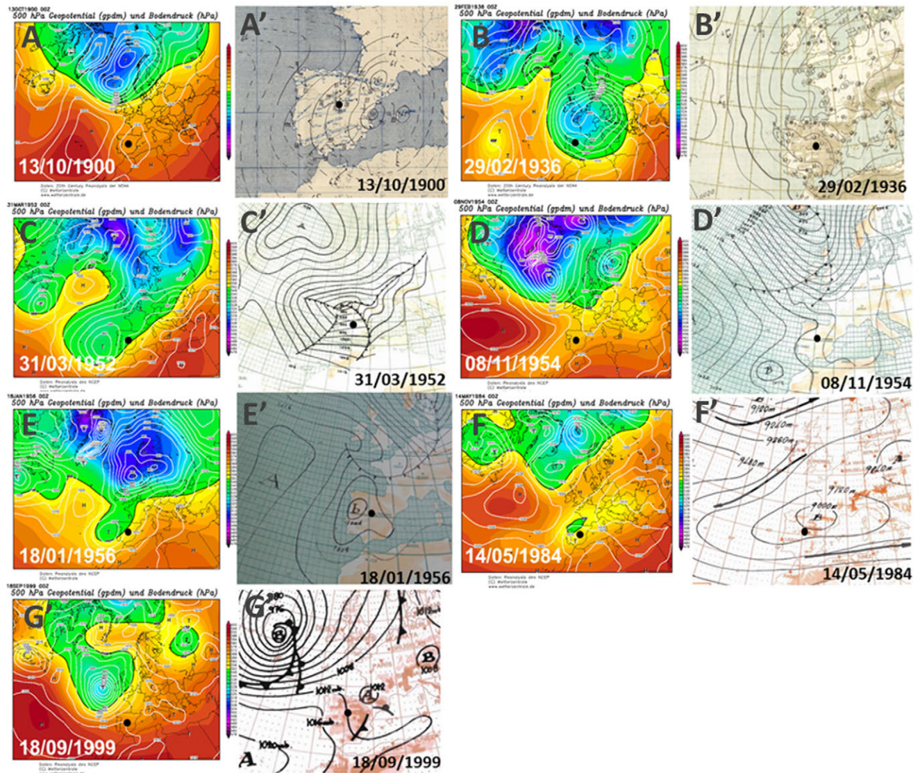
Fig. 7. Synoptic situation (at surface level and 500 hPa level) related with dated flash flood events at the central part of Spain: (A 500 hPa level; A' surface level-hereafter) 13/10/1900 (WZ): zonal atmospheric circulation with low air pressure on the east of the Iberian Peninsula – advection at the study site W; (B) 29/02/1936 (TM) Mixed Central Europe, depth low air pressure on France – advection N; (C) 31/03/1952 (HNZ) meridional atmospheric circulation with depth low air pressure on the NW of the Iberian Peninsula – advection NW; (D) 08/11/1954 (WZ) zonal atmospheric circulation with a trough on the Iberian Peninsula, polar air masses – advection NW; (E) 18/01/1956 (NWZ) mixed atmospheric circulation with a trough on the Iberian Peninsula – advection W; (F) 14/05/1984 (HFZ) meridional atmospheric circulation with low pressure on the Iberian Peninsula, Atlantic air masses – advection N; (G) 18/09/1999 (TRW) meridional atmospheric circulation with a depth low pressure on Britain, Atlantic air masses – advection W. Maps from http://www.wetterzentrale.de (500 hPa, NCEP Reanalysis data) and the Spanish Meteorological Agency (surface maps; http://www.aemet.es/es/conocermas/fondos_digitales/boletines ).
