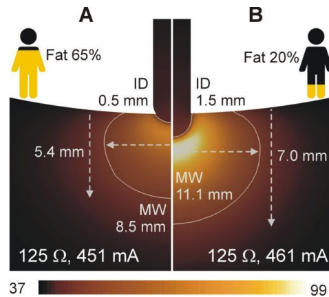
Figure 5. Temperature distributions (scale in ^{\circ}\text{C} ) for two cases showing the same baseline impedance ( 125 \Omega ) despite different insertion depths of the electrode (0.5 mm in (A) vs. 1.5 mm in (B)) and fat percentages in the torso (65% in (A) vs. 20% in (B)). Note that the resultant lesion sizes are different despite identical baseline impedances. The RF current at the middle of the RF pulse (15 s) is 10 mA higher in the case of the largest lesion.
