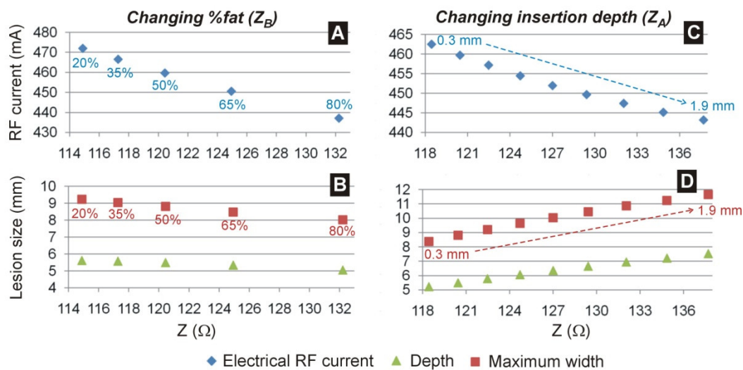
Figure 4. Electrical RF current (at the middle of the RF pulse, 15 s) (A and C) and lesion size (B and D) for different values of baseline impedance. While in panels (A) and (B) the baseline impedance varied due to the 'remote' impedance, specifically the percentage of fat around the organs (from 20 to 80%), in panels (C) and (D) the baseline impedance varied due to the 'local' impedance, specifically the electrode insertion depth in the myocardium (from 0.3 to 1.9 mm).
