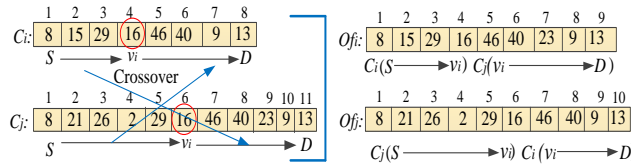
Fig. 7. Crossover operation and two new offspring
