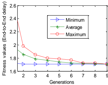
Fig.22.Comparison of maximum, average, and minimum fitness values
