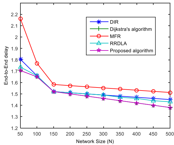
Fig. 26. Comparison of end-to-end delay with varying network size.
