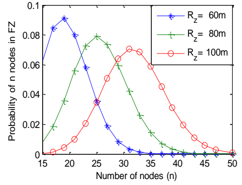
Fig. 11. Probability of number of nodes in FZ with different transmission range
