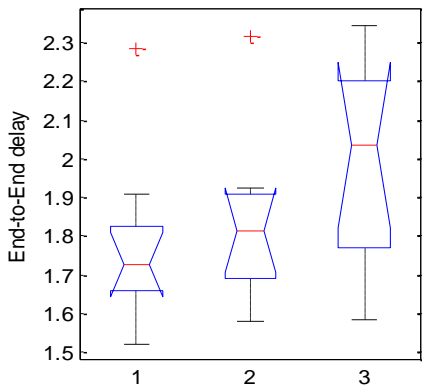
Fig. 27.ANOVA graph
